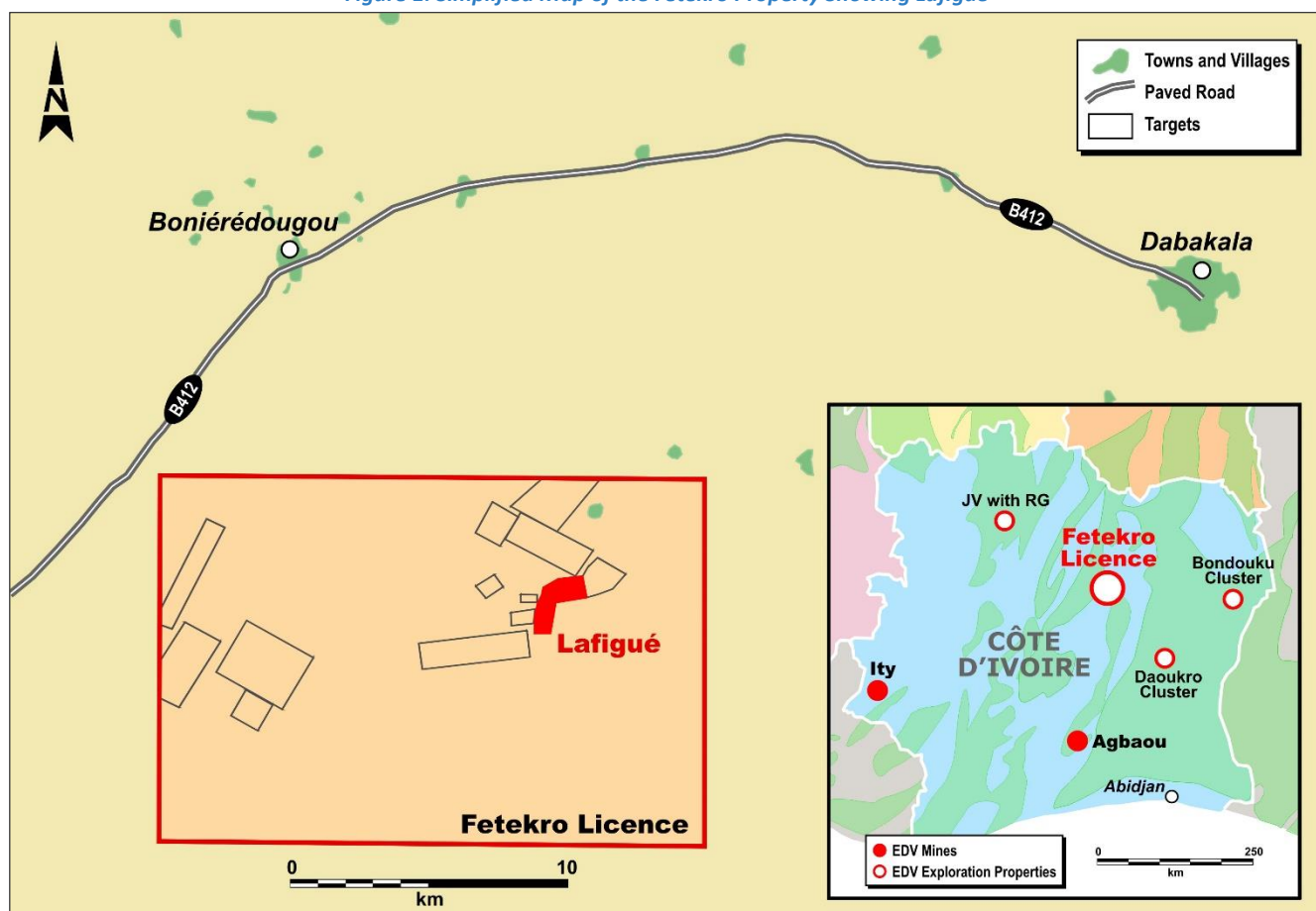
Figure 1: Simplified Map of the Fetekro Property Showing Lafigué
