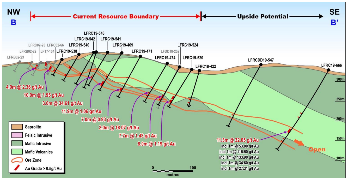
Figure 4: Lafigué North Cross-Section (Western part)
