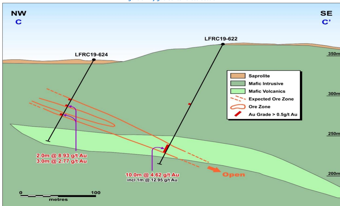
Figure 5: Lafigué Center Cross-Section
