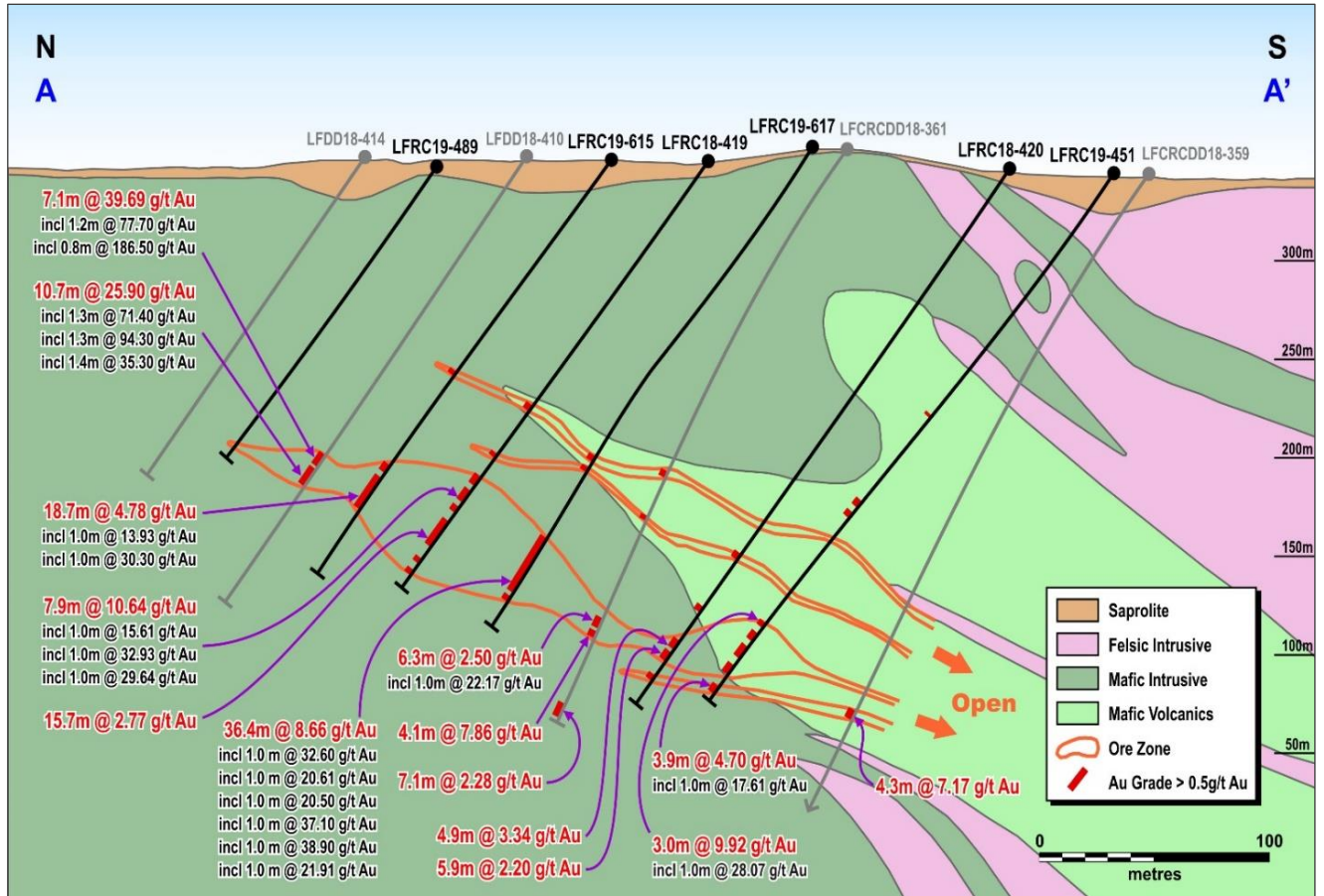
Figure 3: Lafigué North Cross-Section (Eastern part)
