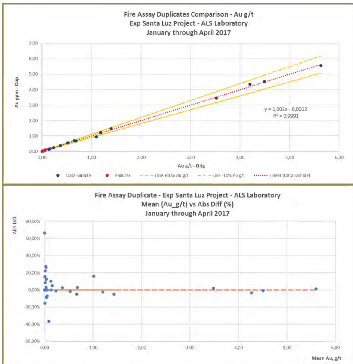
Figure 11-5: Fire Assay Duplicates Performance for Gold (2017)
