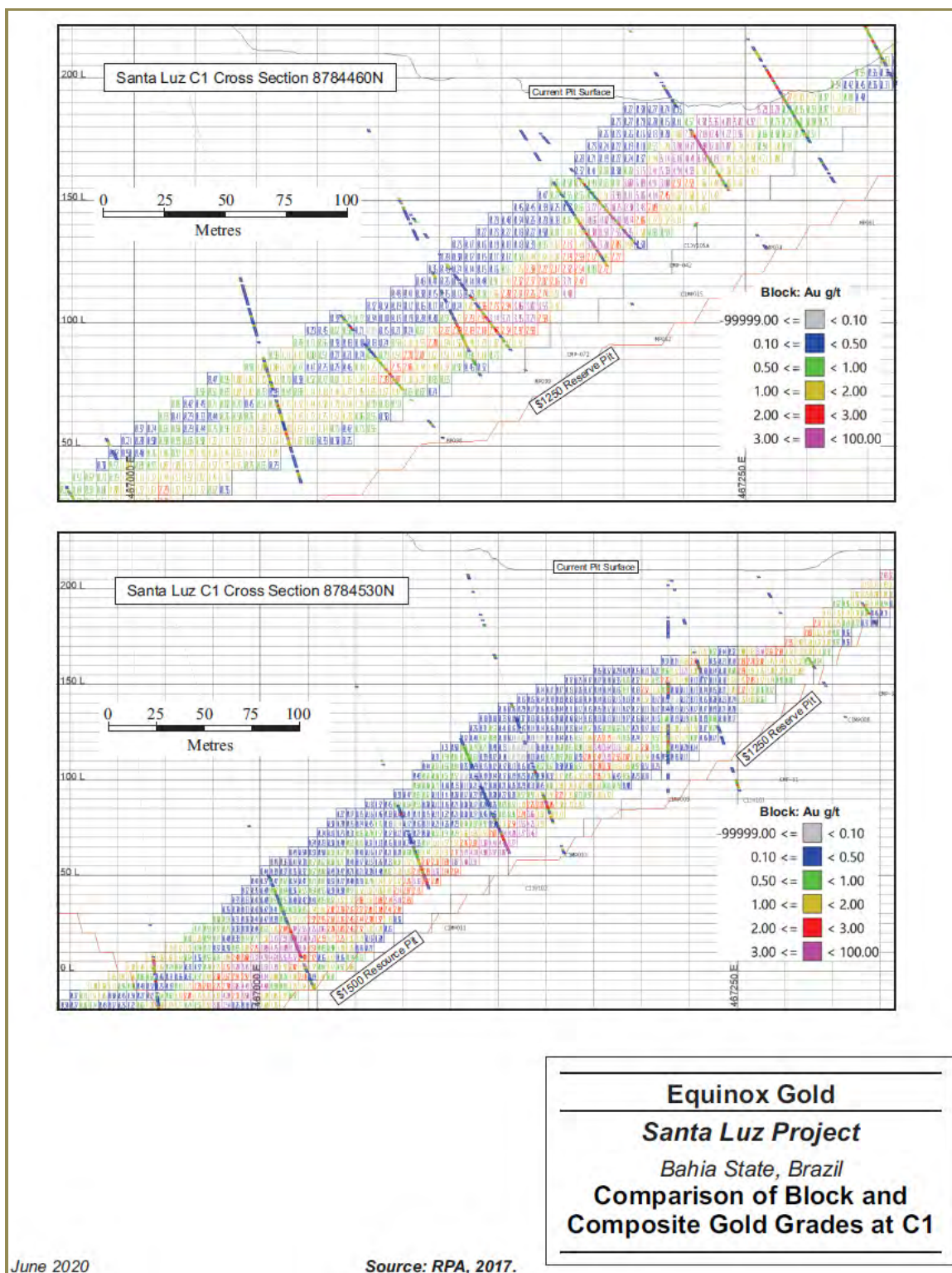
Figure 14-24: Comparison of Block and Composite Gold Grades at C1
