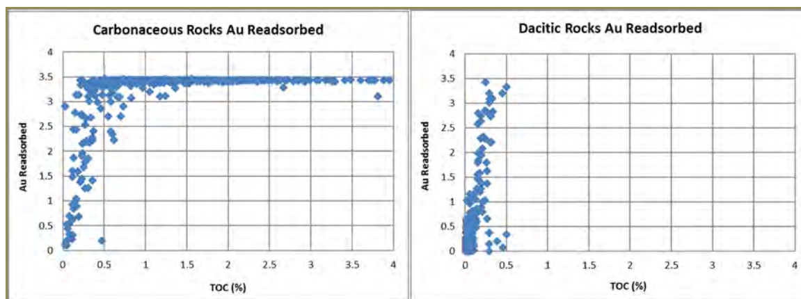
Figure 7-8: Carbonaceous and Dacitic Rocks TOC vs. Au Re-Adsorbed
