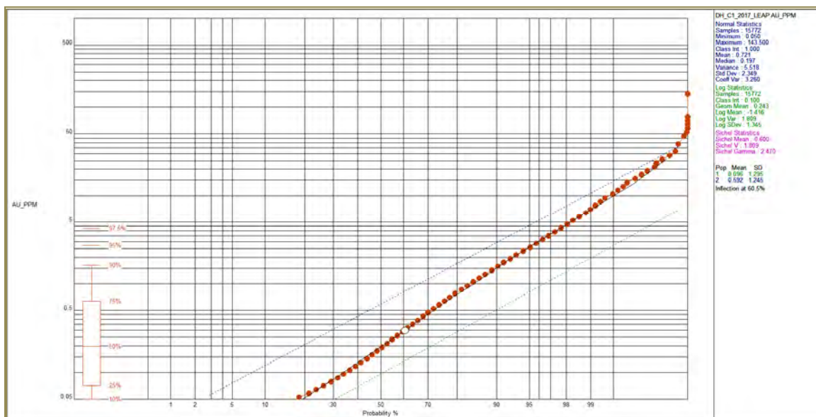
Figure 14-2: C1 Grade Shell Modelling Cut-Off Curve (0.1 g/t Au)
