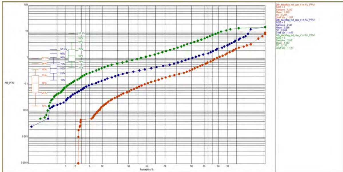
Figure 14-7: C1 Probability Plot of Gold for Three Indicator Zones
