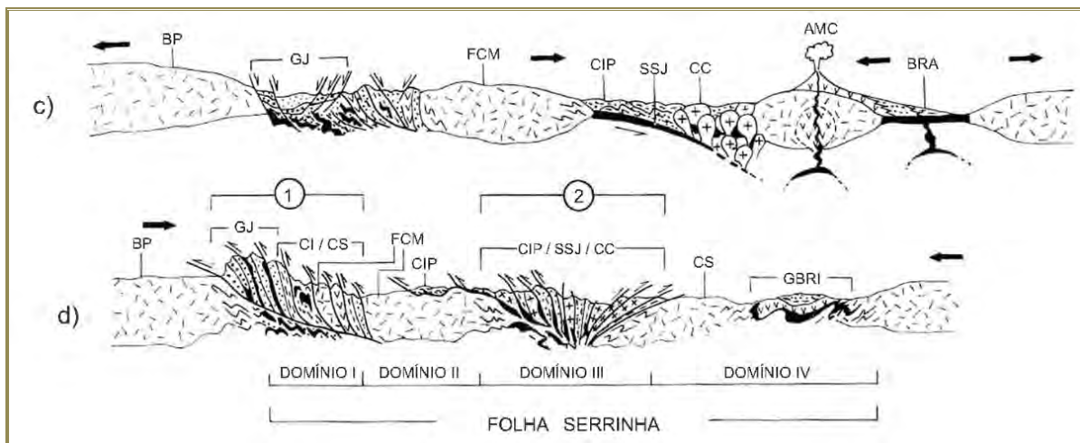
Figure 7-1: Regional Geology—Rio Itapicuru Greenstone Belt
