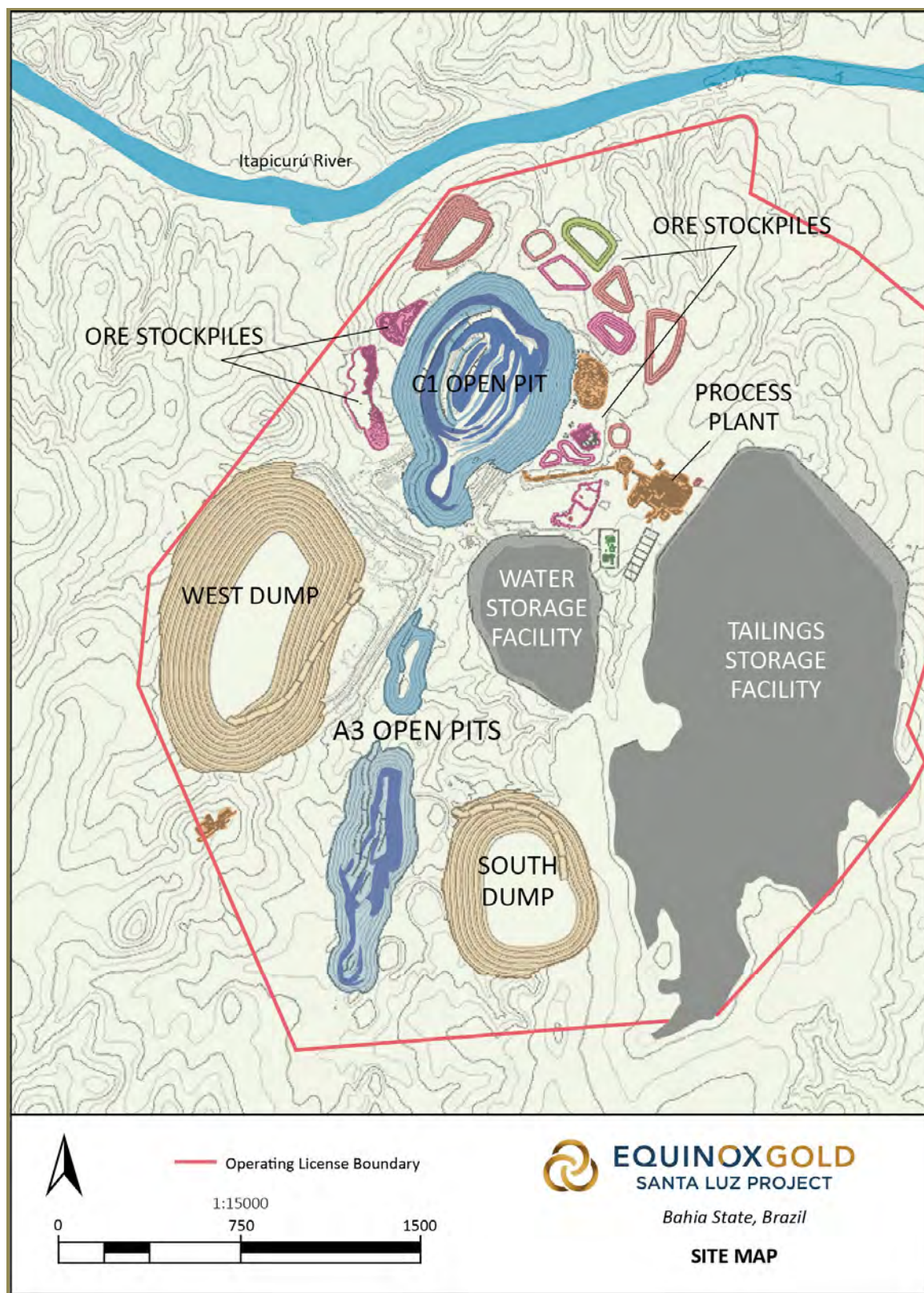
Figure 1-4: Site Infrastructure
