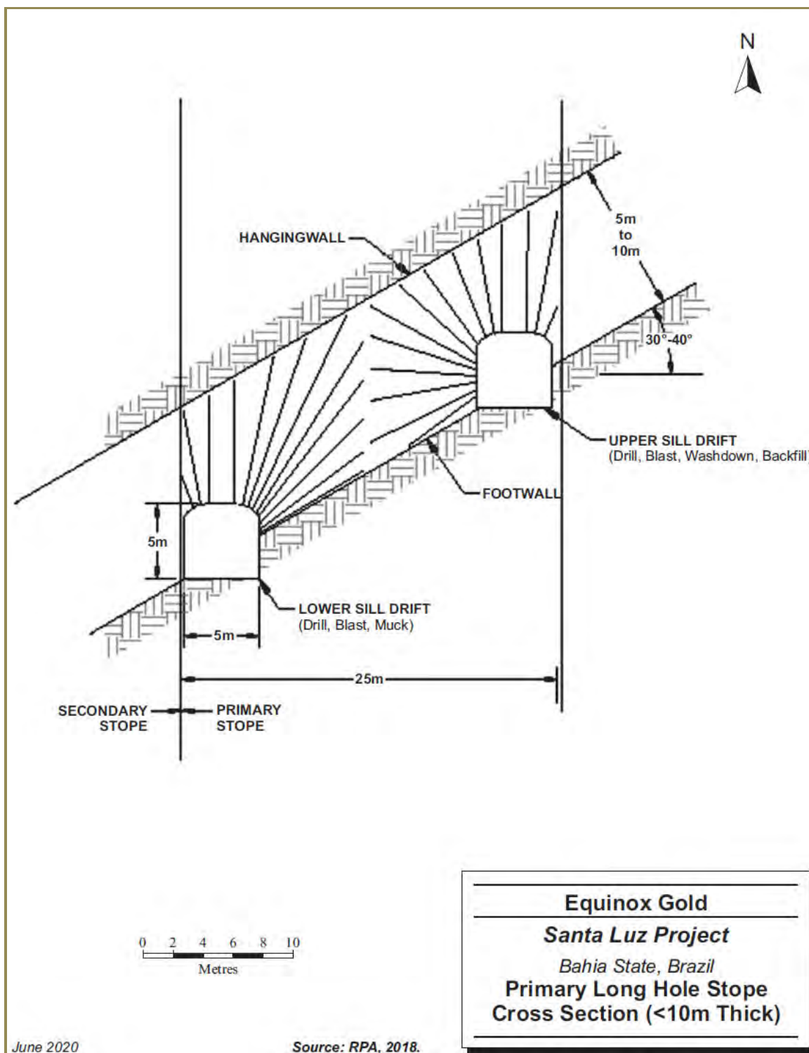
Figure 24-8: Primary Long Hole Stope Cross Section (<10 m Thick)
