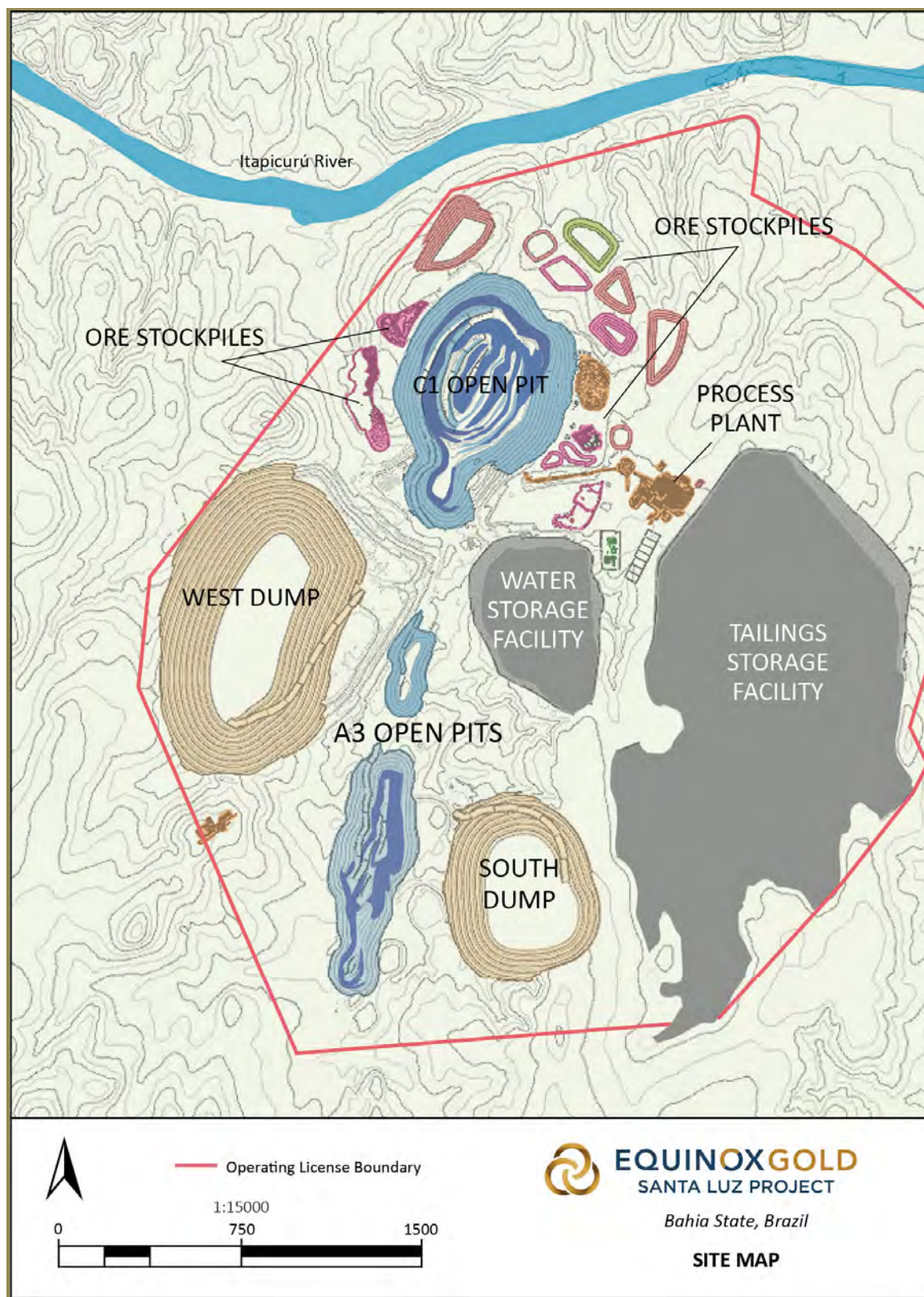
Figure 18-1: Site Infrastructure
