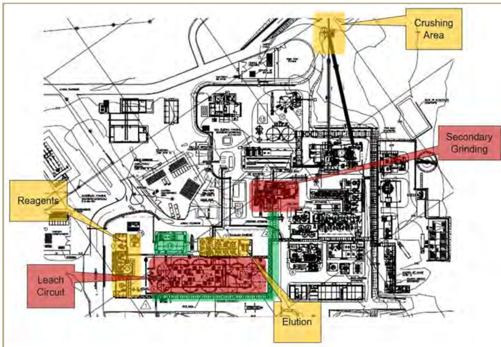
Figure 1-2: Process Plant General Arrangement
