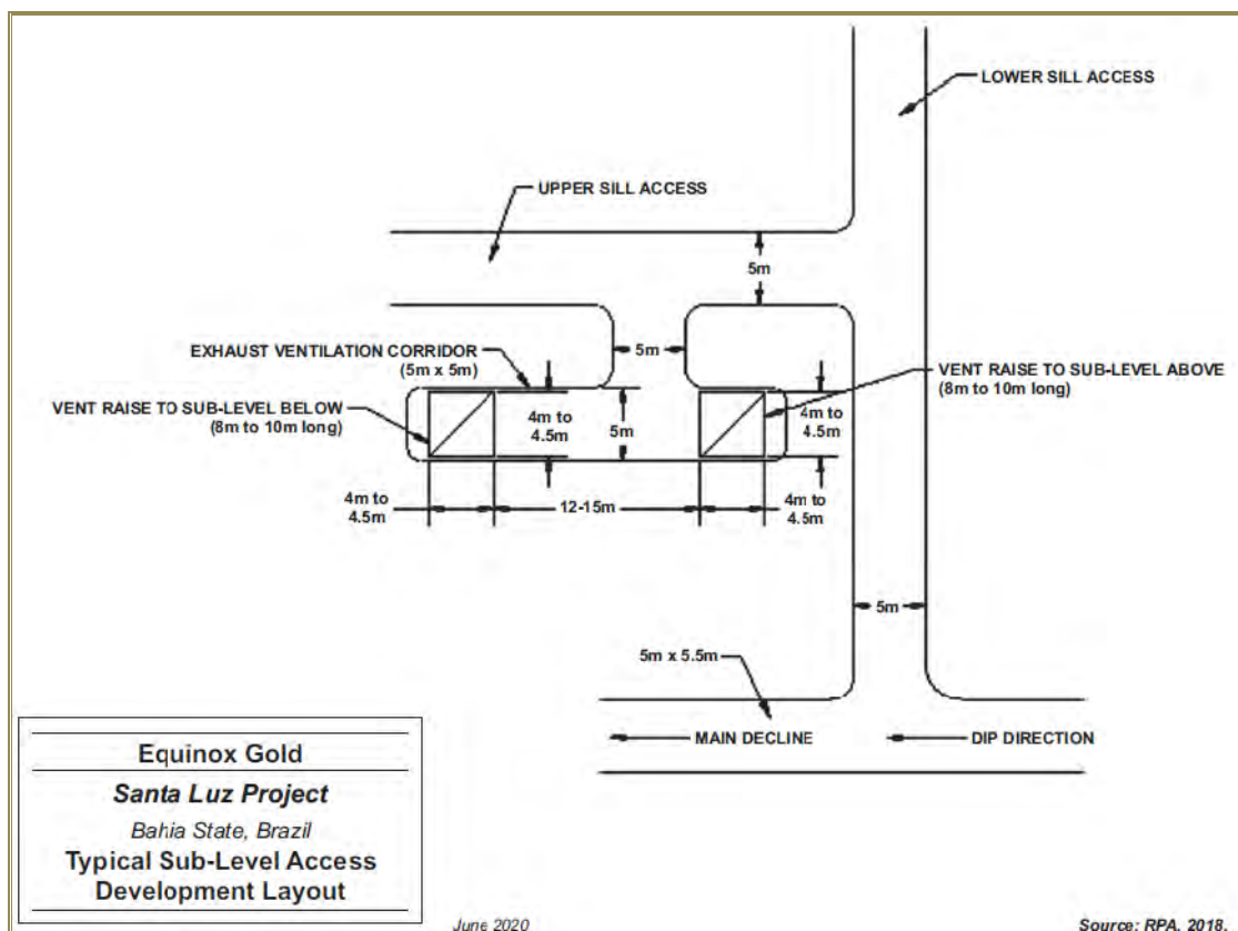
Figure 24-5: C1 Underground Typical Sub-Level Access Development Layout
