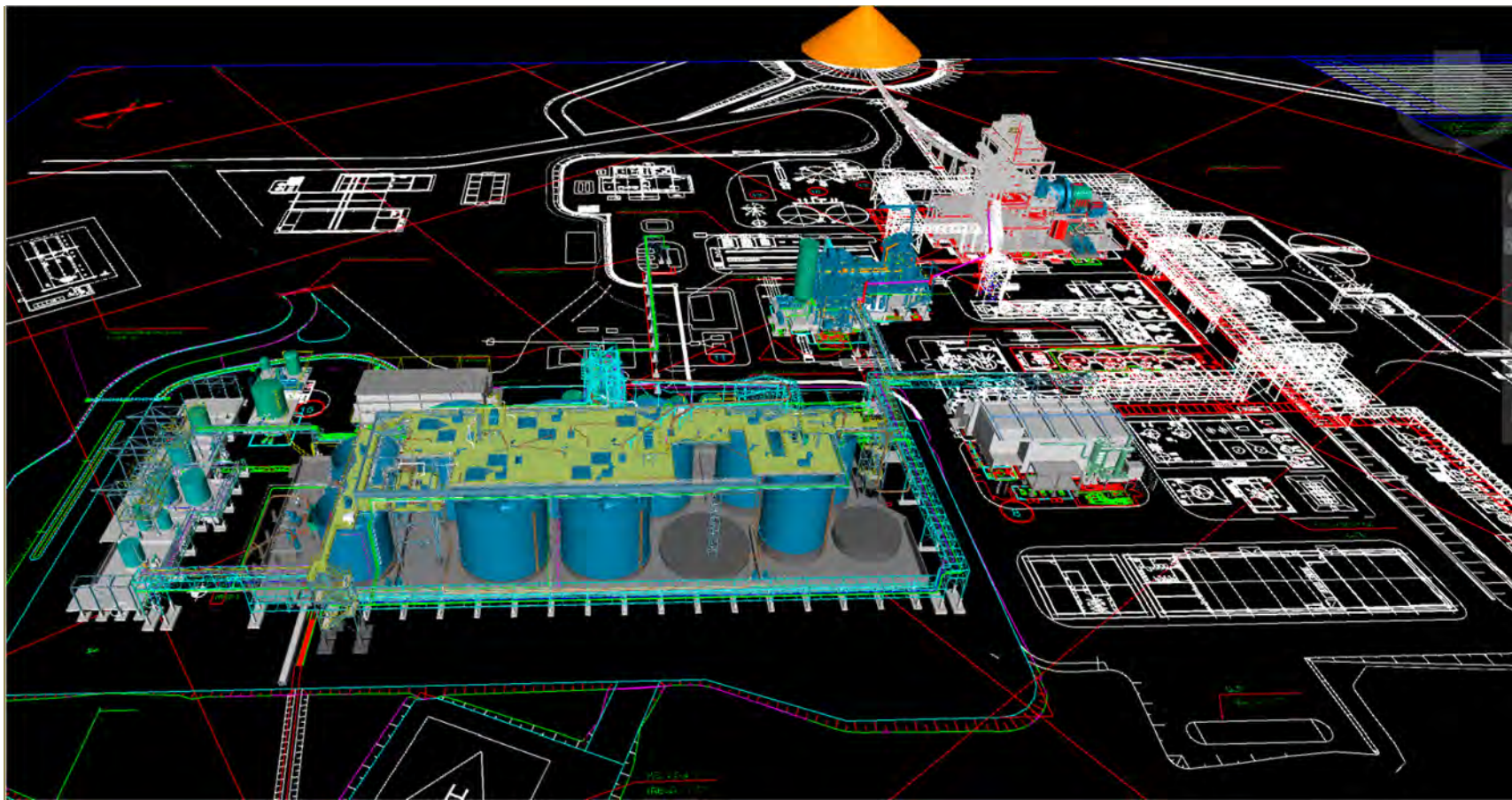
Figure 1-3: Process Plant 3D Isometric View
