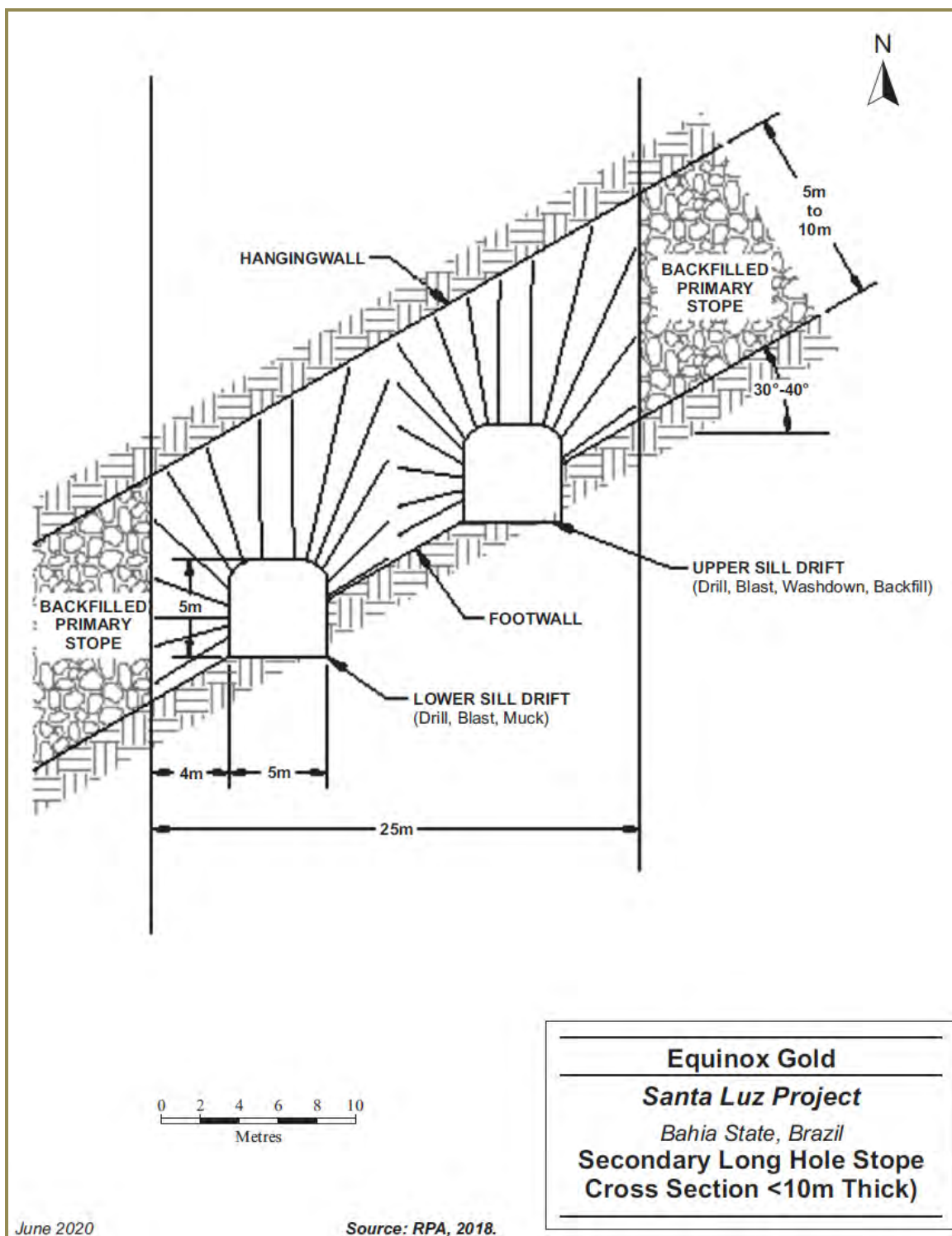
Figure 24-9: Secondary Long Hole Stope Cross Section (<10 m Thick)
