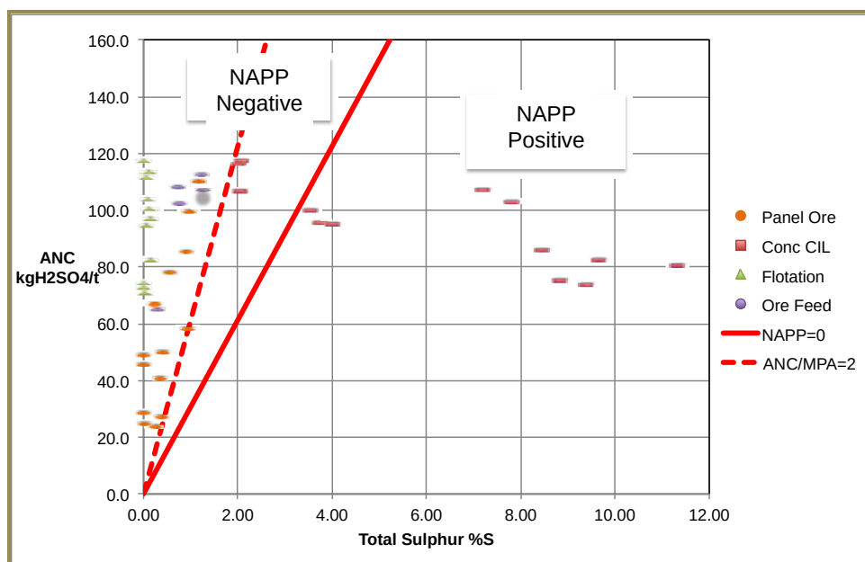
Figure 20-4: Acid Base Account Plot
