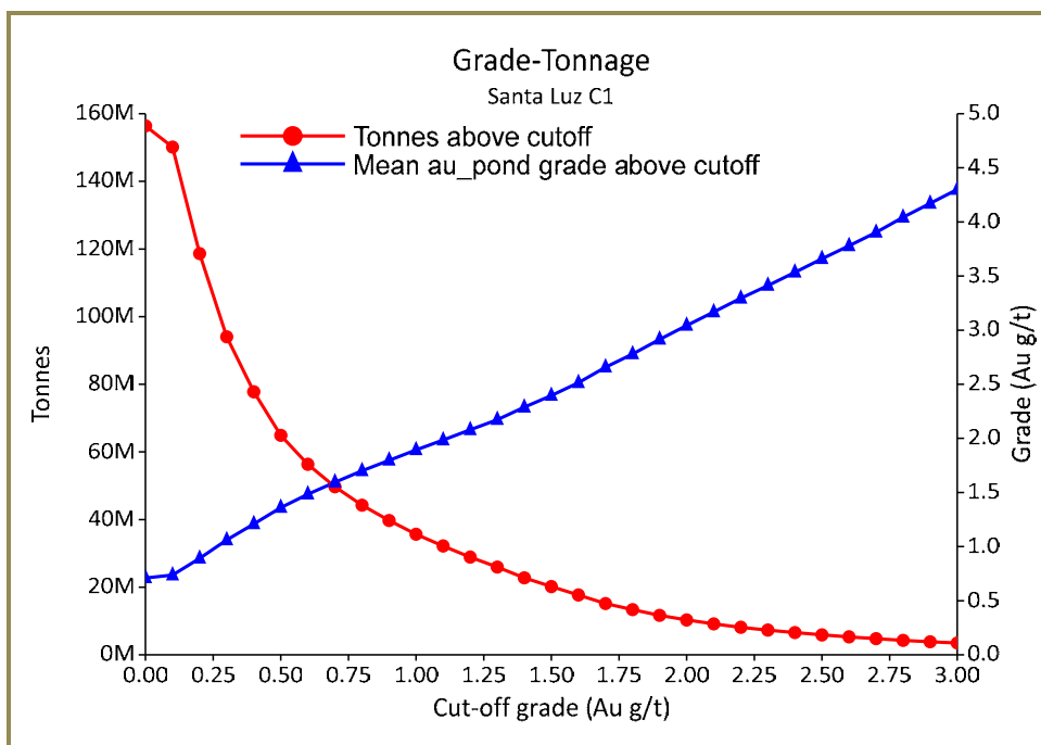
Figure 14-30: C1 Mineral Resource Tonnes and Grade at Various Cut-Off Grades
