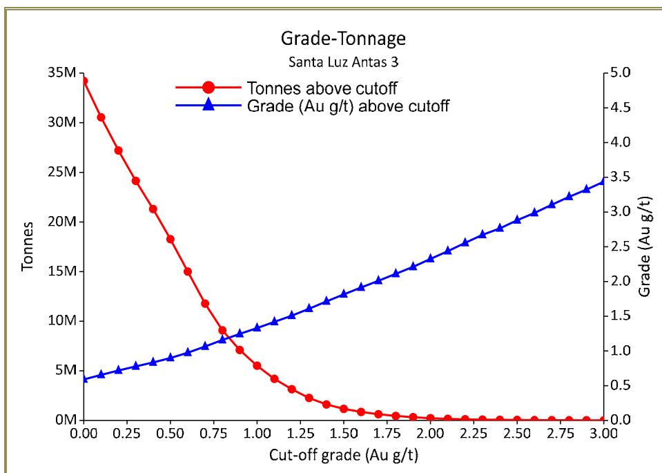
Figure 14-31: Antas 3 Mineral Resource Tonnes and Grade at Various Cut-Off Grades
