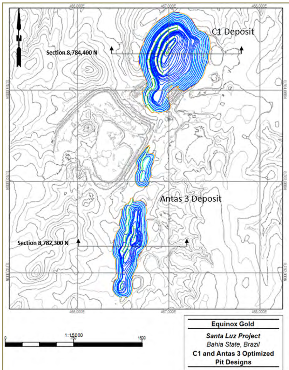
Figure 16-1: C1 and Antas 3 Optimized Pit Designs
