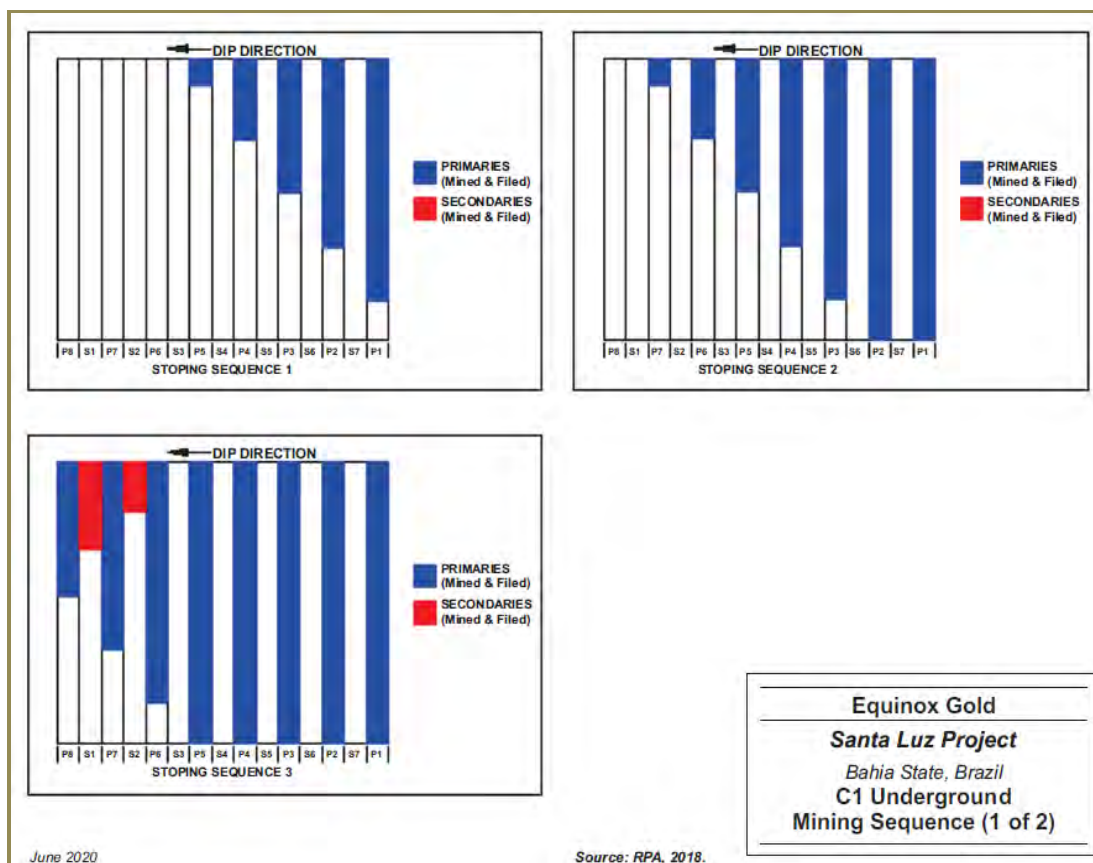
Figure 24-11: C1 Underground Mining Sequence (1 of 2)
