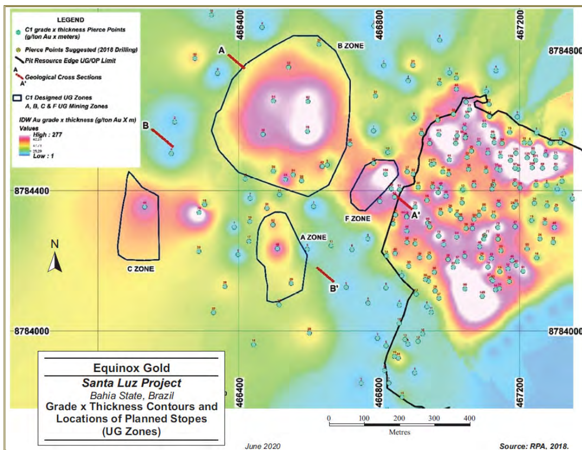
Figure 24-2: C1 Underground Grade x Thickness Contours and Locations of Planned Stopes (Underground Zones)
