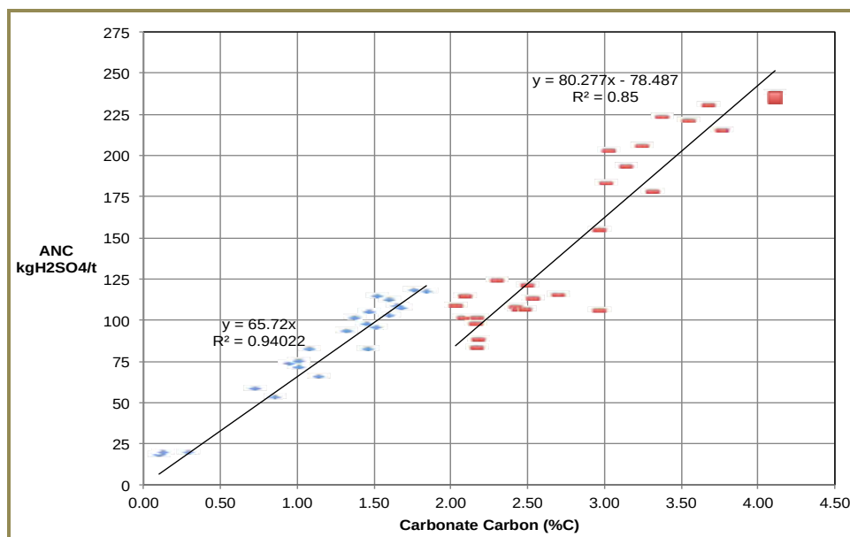
Figure 20-2: Carbonate Carbon and ANC for Ore, Flotation, and Combined Tailings
