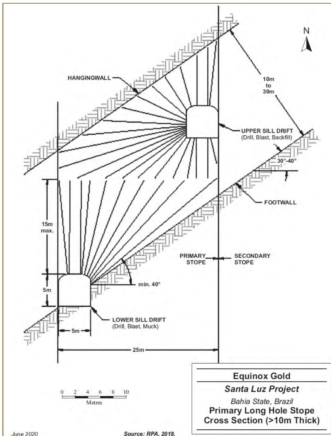
Figure 24-6: Primary Long Hole Stope Cross Section (>10 m Thick)
