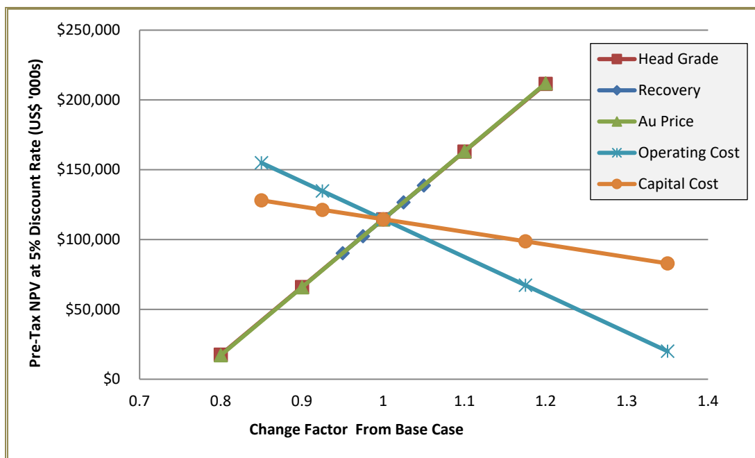
Figure 24-14: C1 Underground Sensitivity Analysis NPV Base Case
