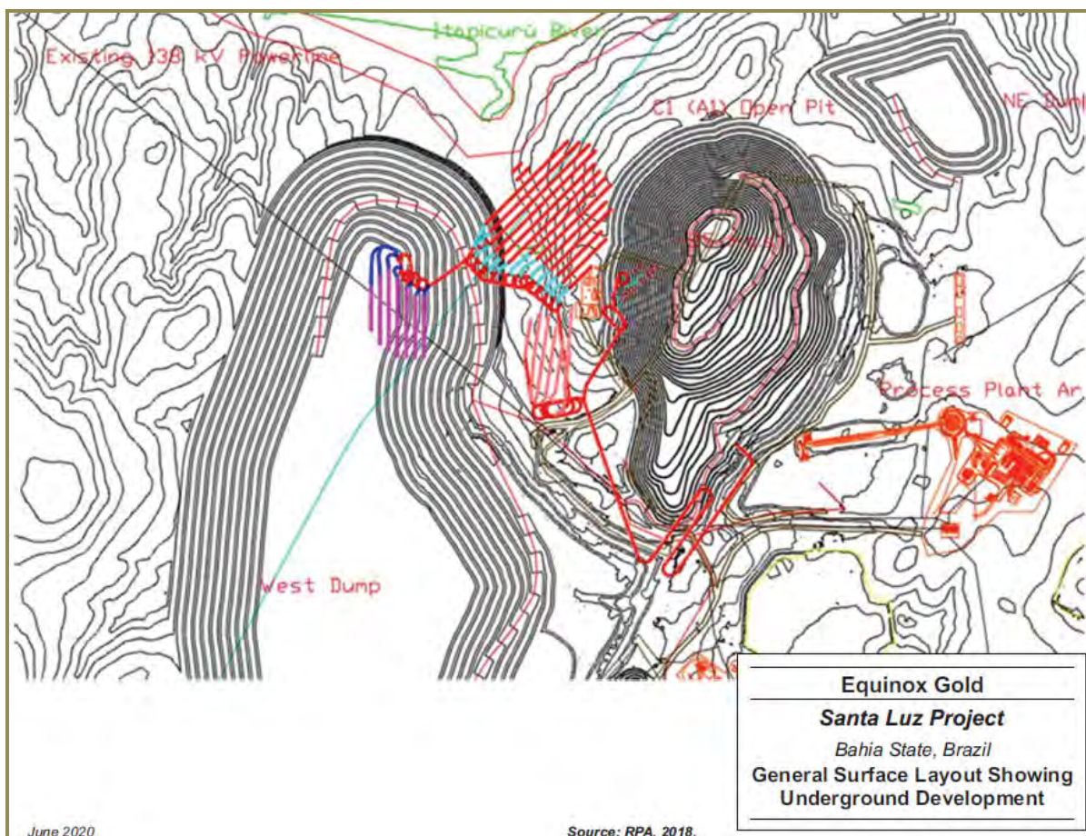
Figure 24-13: General Surface Layout Showing the C1 Underground Development
