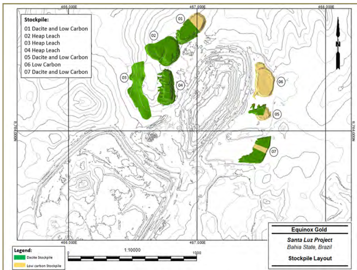
Figure 15-1: Stockpile Layout
