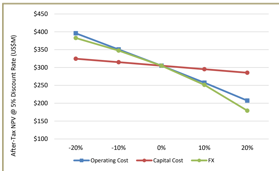
Figure 1-6: Operating Cost, Capital Cost, and Foreign Exchange Sensitivity Analysis on After-Tax NPV
