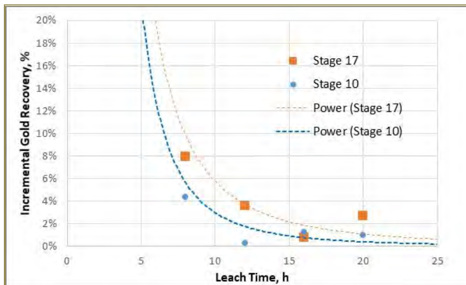
Figure 13-2 Comparison of Incremental Recovery by Tank for Stage 10 and Stage 17
