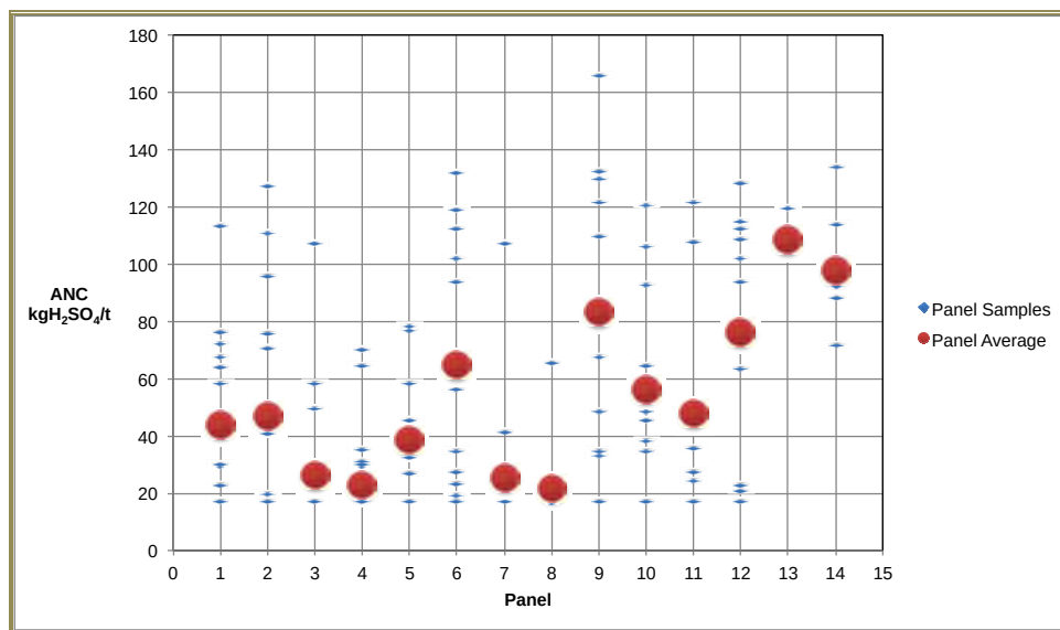
Figure 20-3: Mine Panel Calculated ANC (ANC cal )
