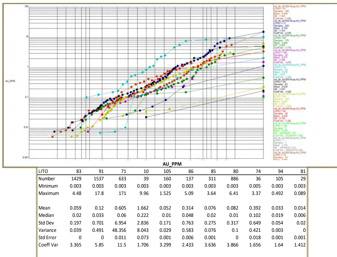
Figure 14-15: Antas 2 Au Probability Plot vs. Lithology
