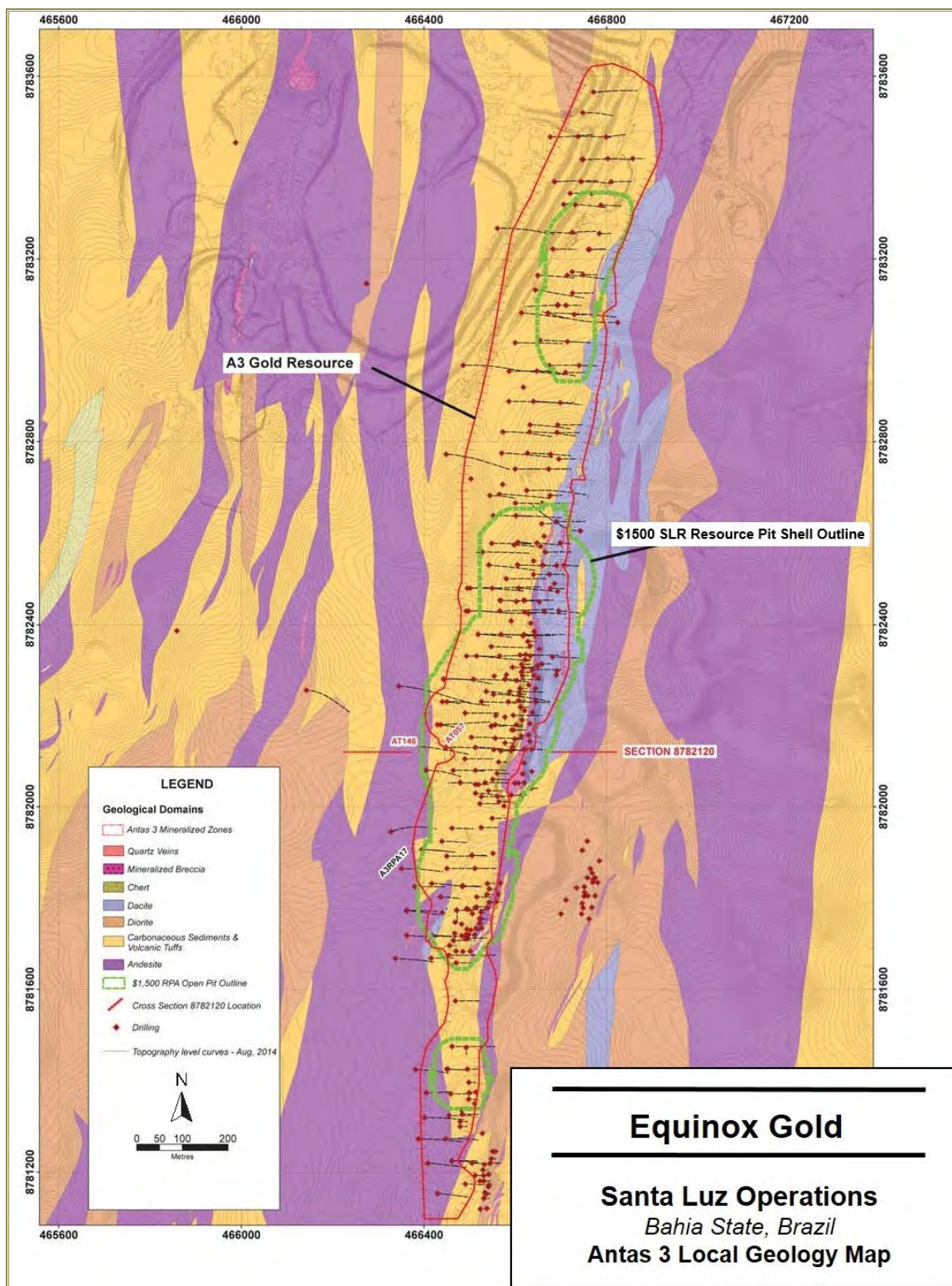
Figure 7-4: Santa Luz Antas 3 Local Geology
