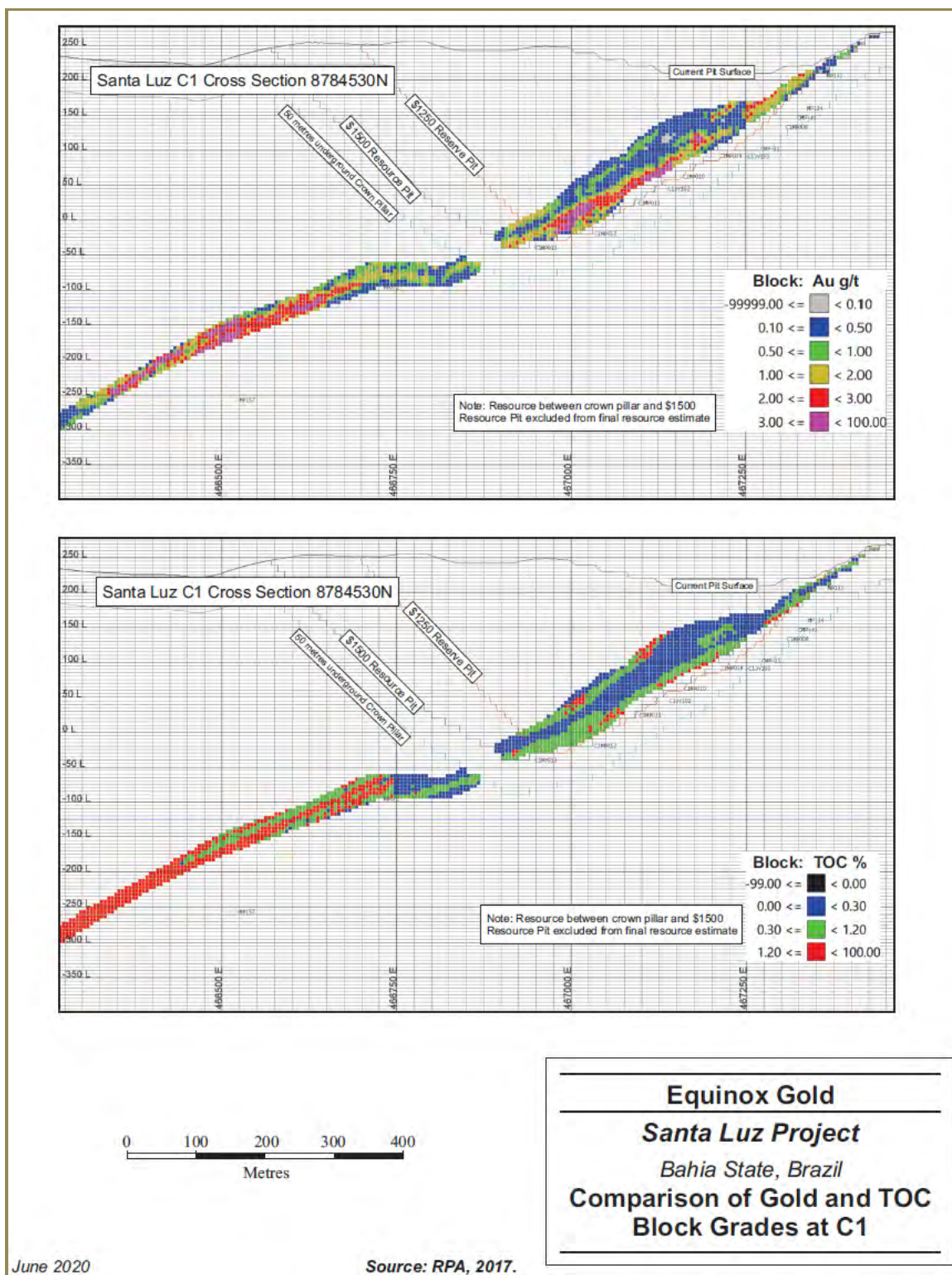
Figure 14-25: Comparison of Gold and TOC Block Grades at C1
