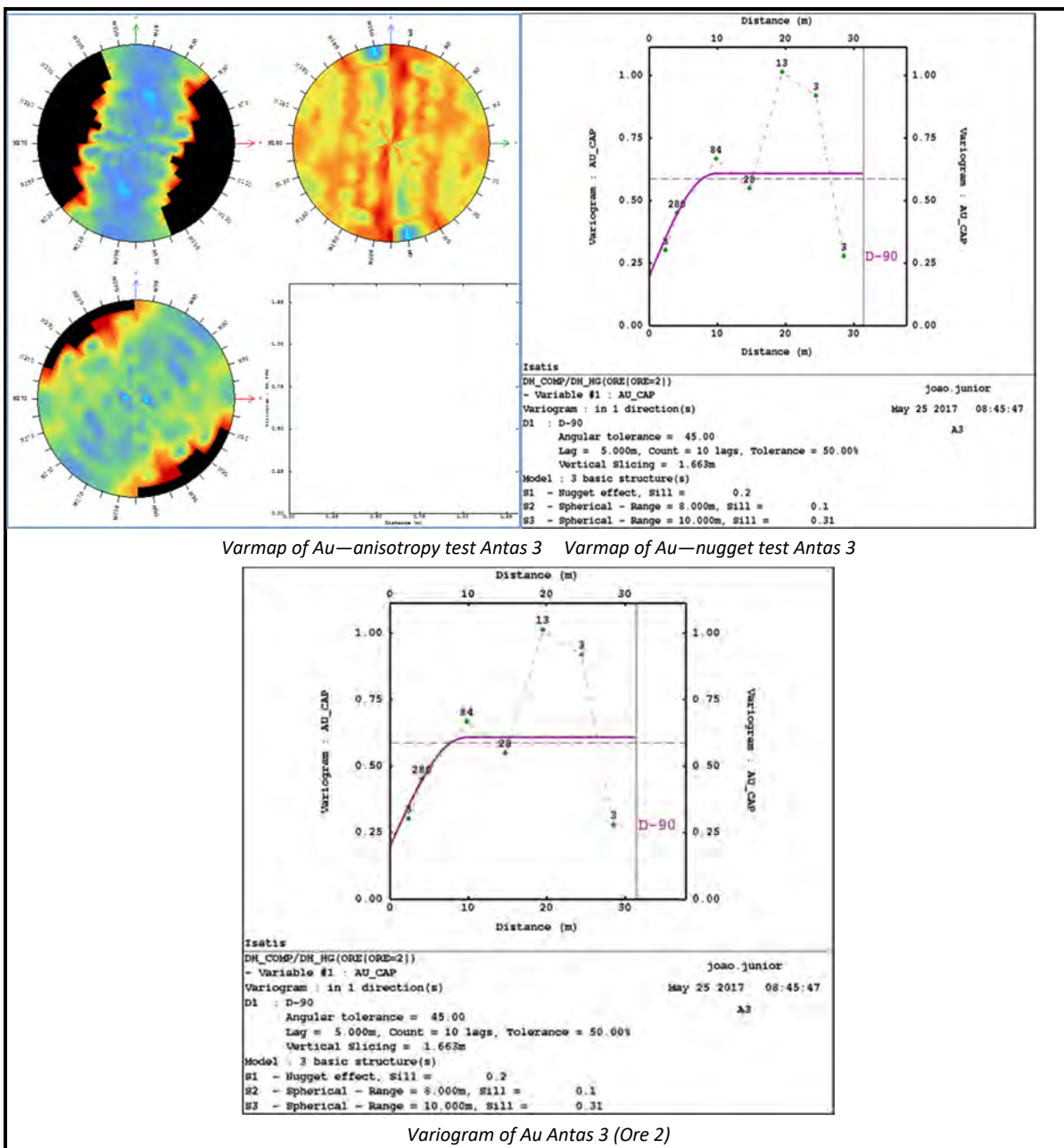
Figure 14-21: Variogram Model at Antas 3
