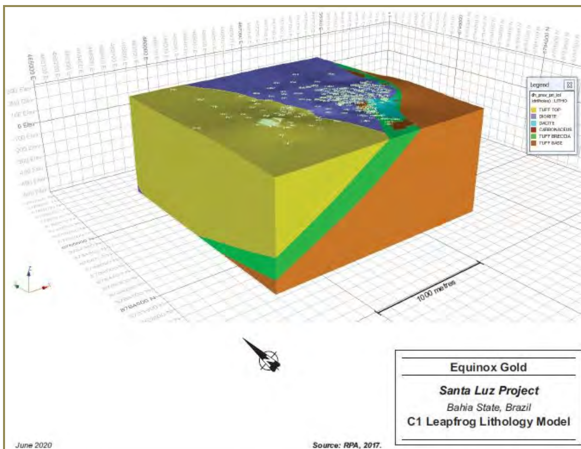
Figure 14-1: C1 Leapfrog Lithology Model
