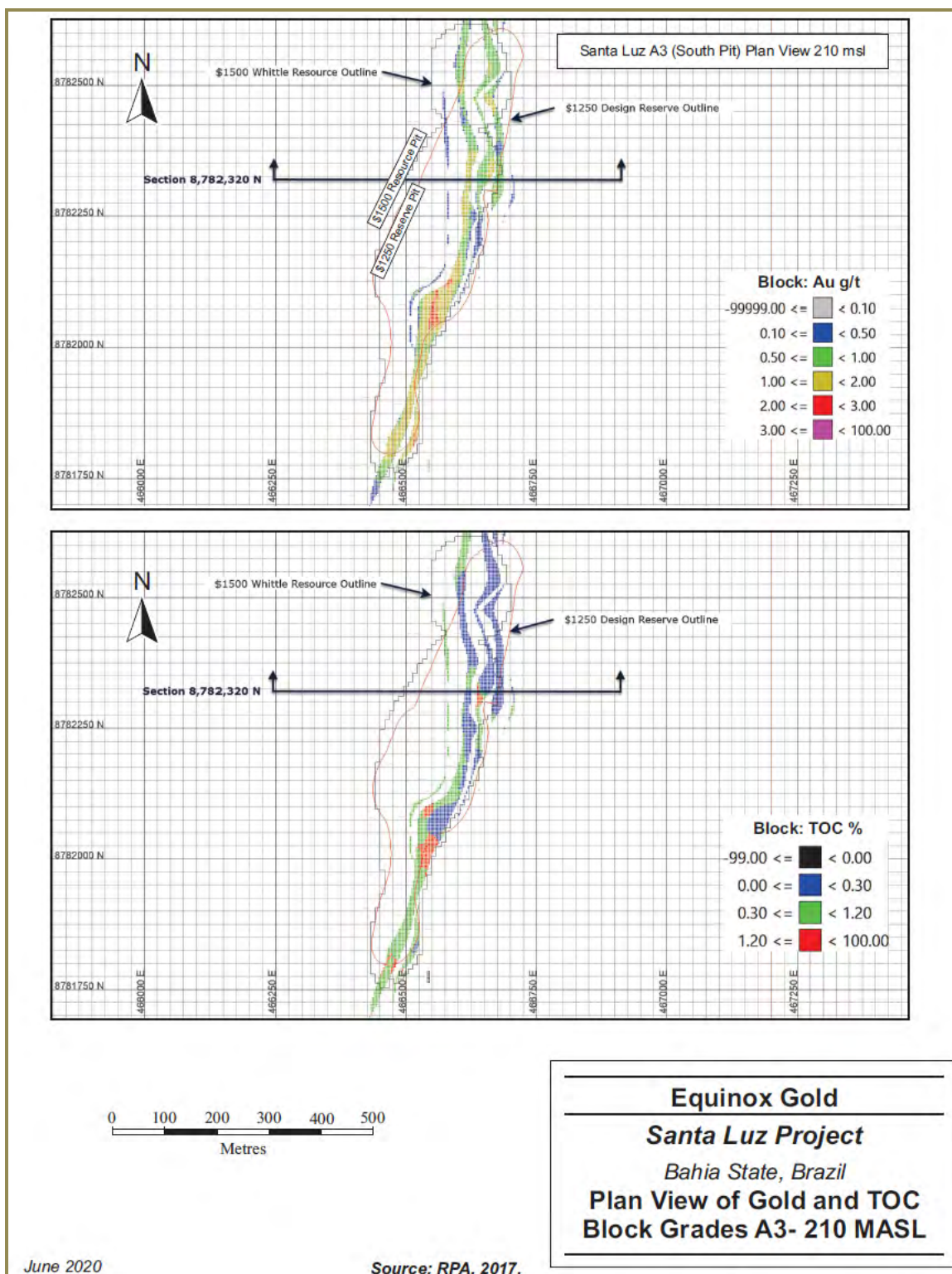
Figure 14-26: Plan View of Gold and TOC Block Grades Antas 3—210 mASL
