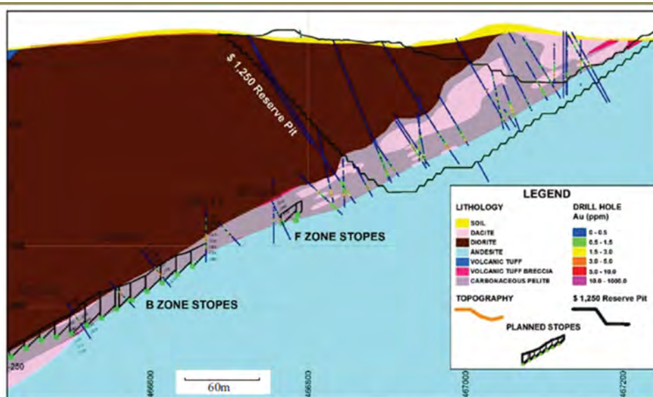
Underground Resource Geologic Cross Section A-A'
