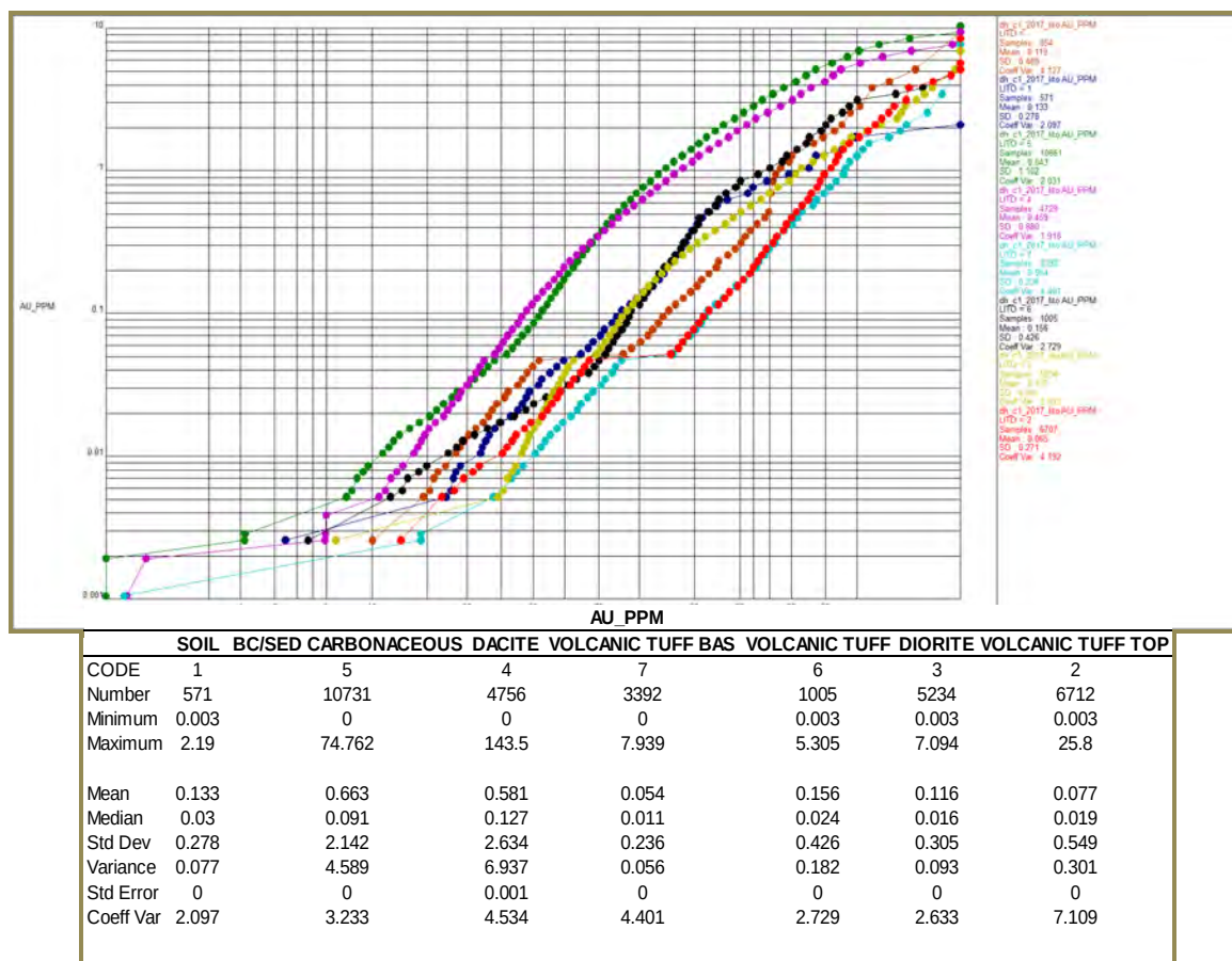
Figure 14-14: C1 Au Probability Plot vs. Lithology
