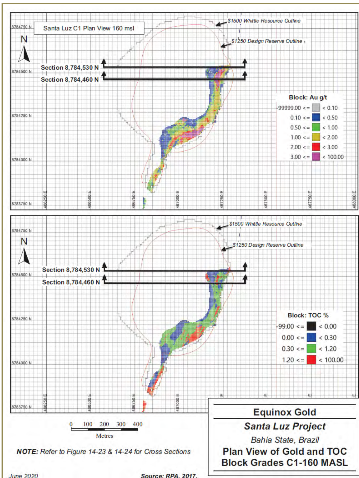
Figure 14-23: Plan View of Gold and TOC Block Grades C1—160 mASL
