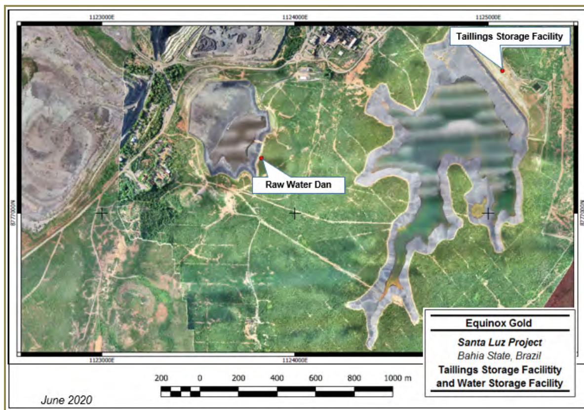
Figure 18-2: Tailings and Water Storage Facilities
