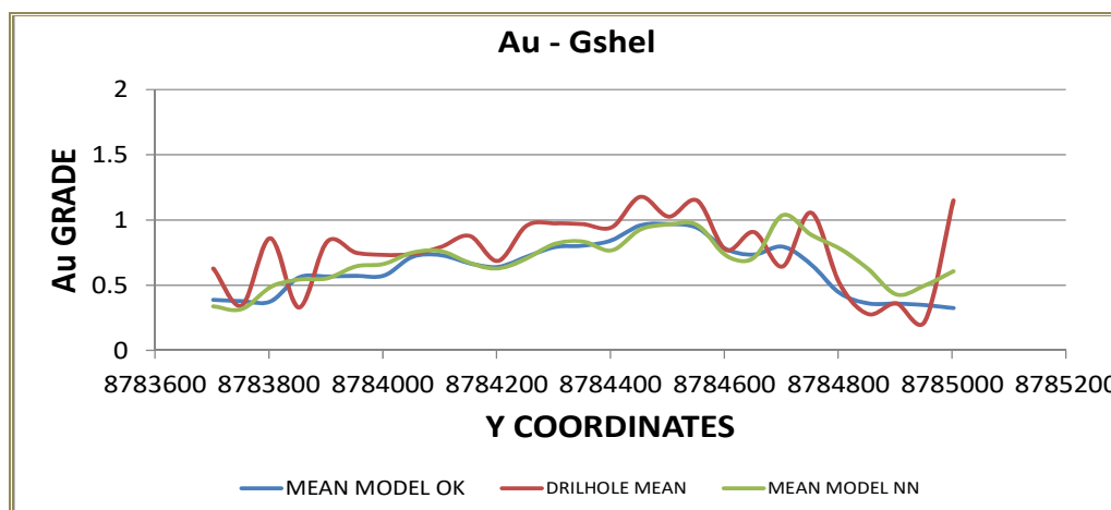
Figure 14-28: Drift Analysis of C1 Grade Shell Block Estimates vs. NN Composite
