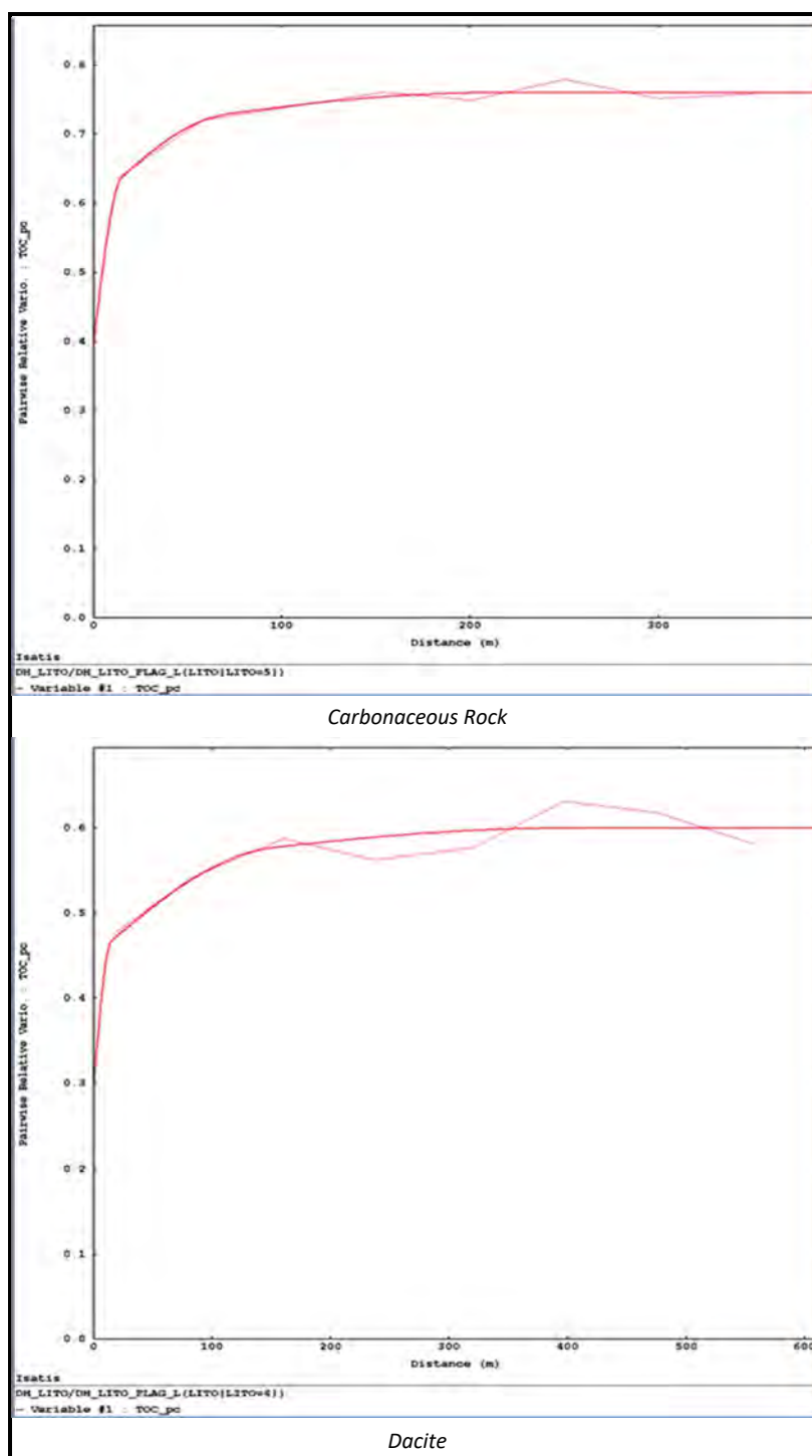
Figure 14-20: Variogram of TOC—Carbonaceous Rock and Dacite At C1
