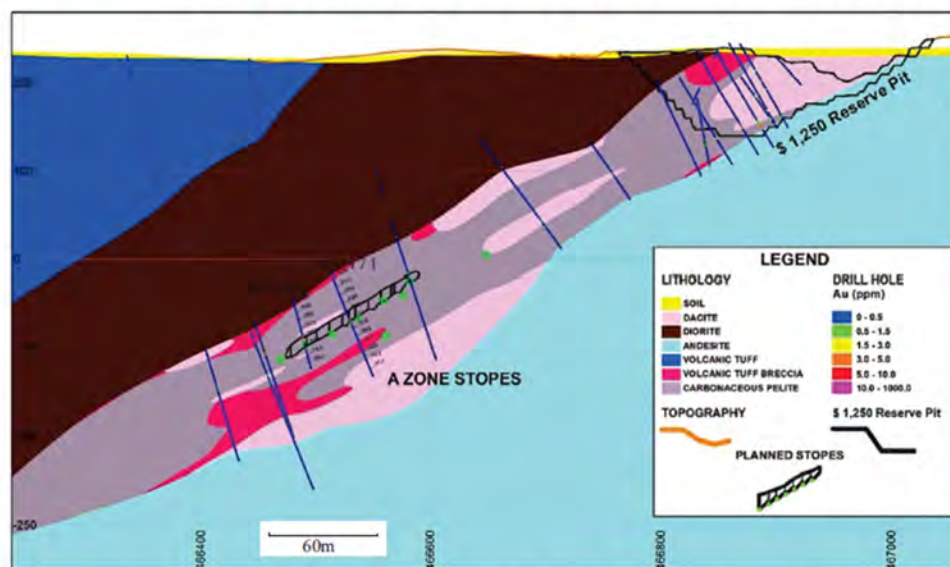
Underground Resource Geologic Cross Section B-B'
