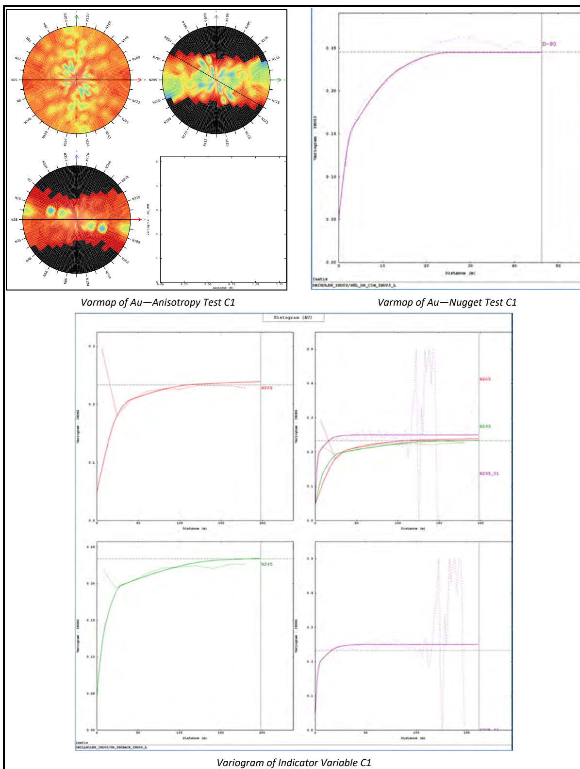
Figure 14-18: Variogram Model at C1
