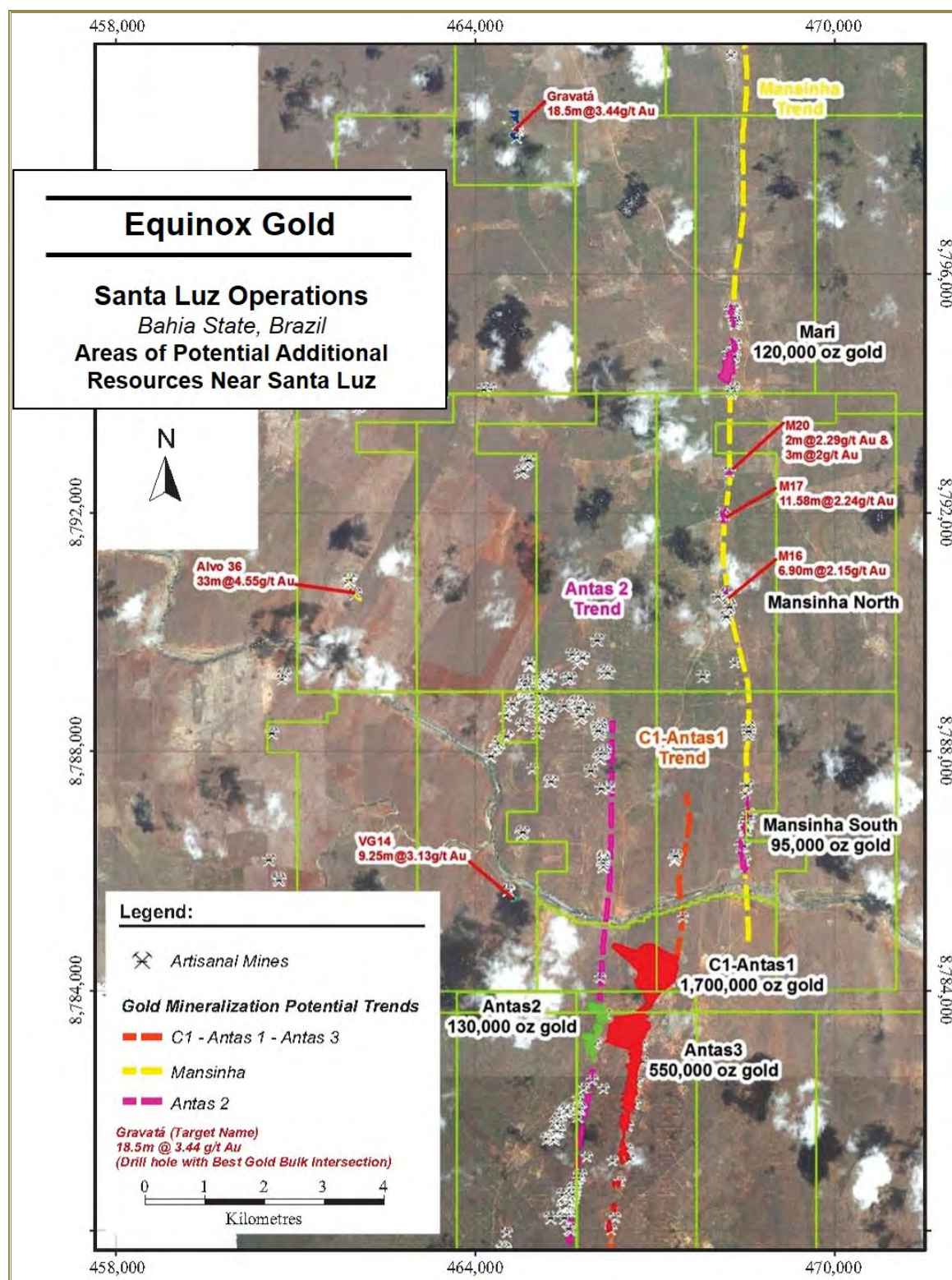
Figure 7-12: Areas of Potential Additional Resources Near Santa Luz
