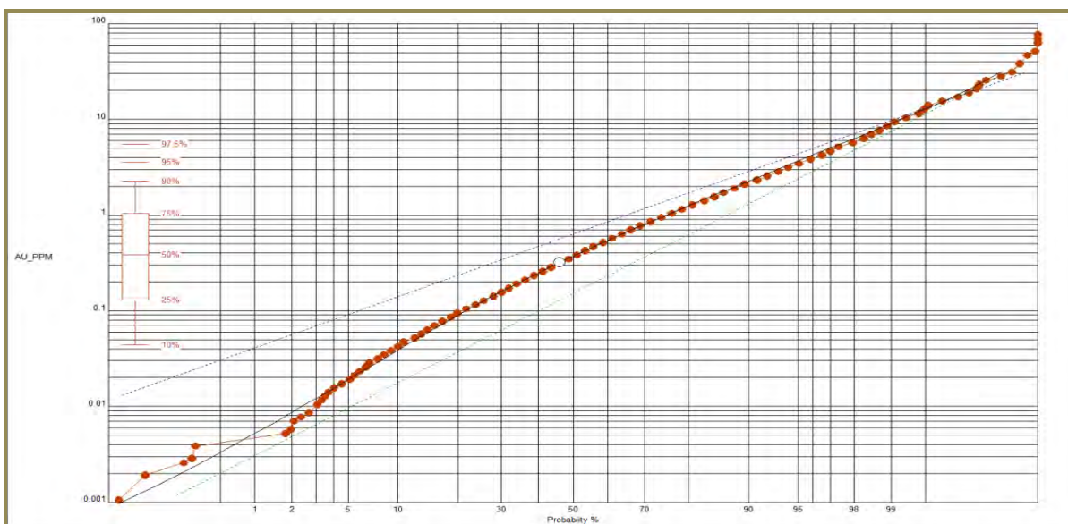
Figure 14-4: C1 Probability Plot Cut-off 0.30 g/t Au
