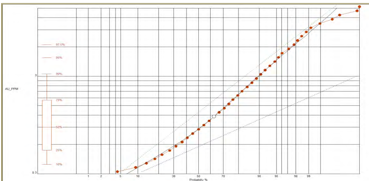
Figure 14-5: C1 Probability Plot Cut-Off 0.60 g/t Au
