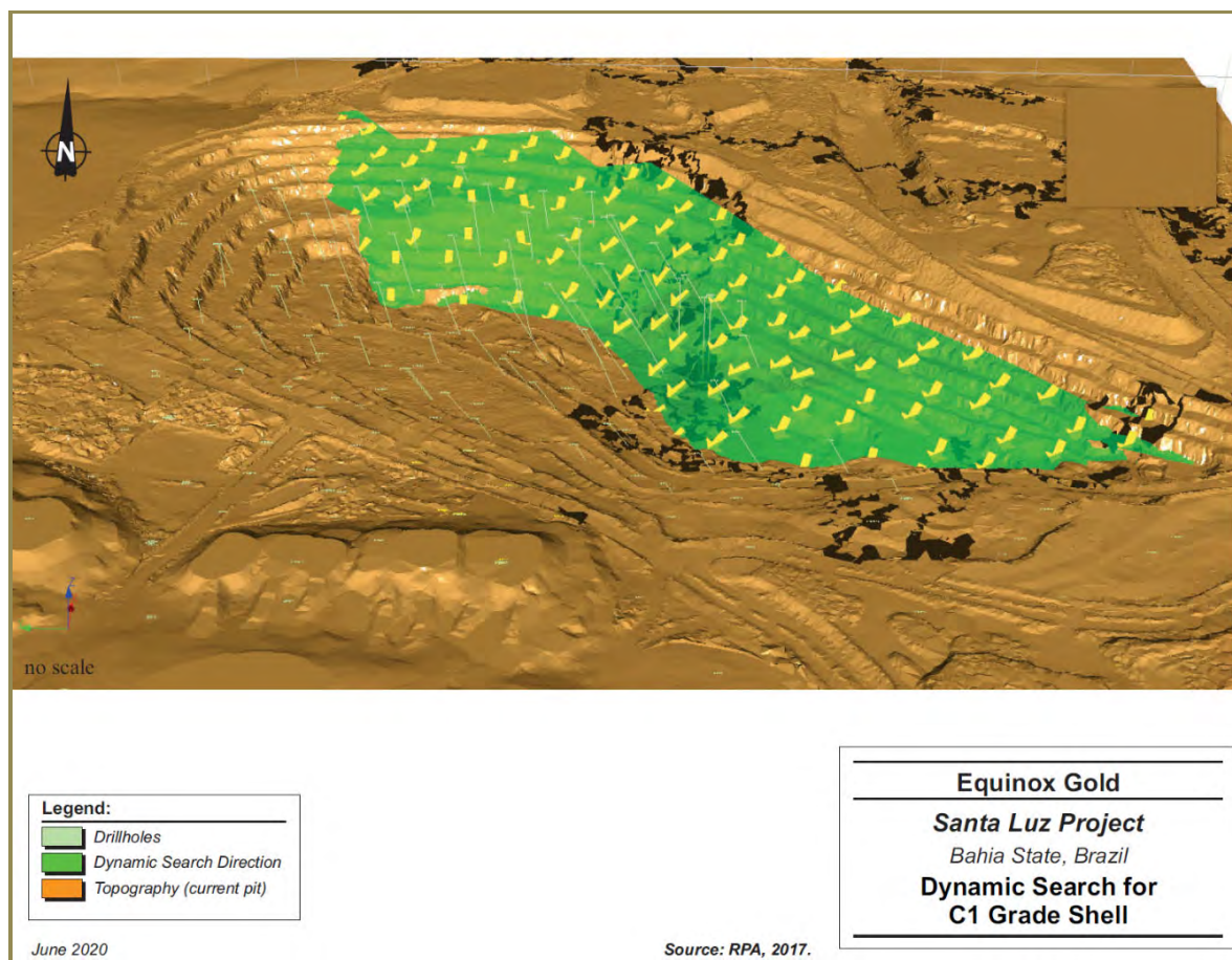
Figure 14-22: Dynamic Search for C1 Grade Shell
