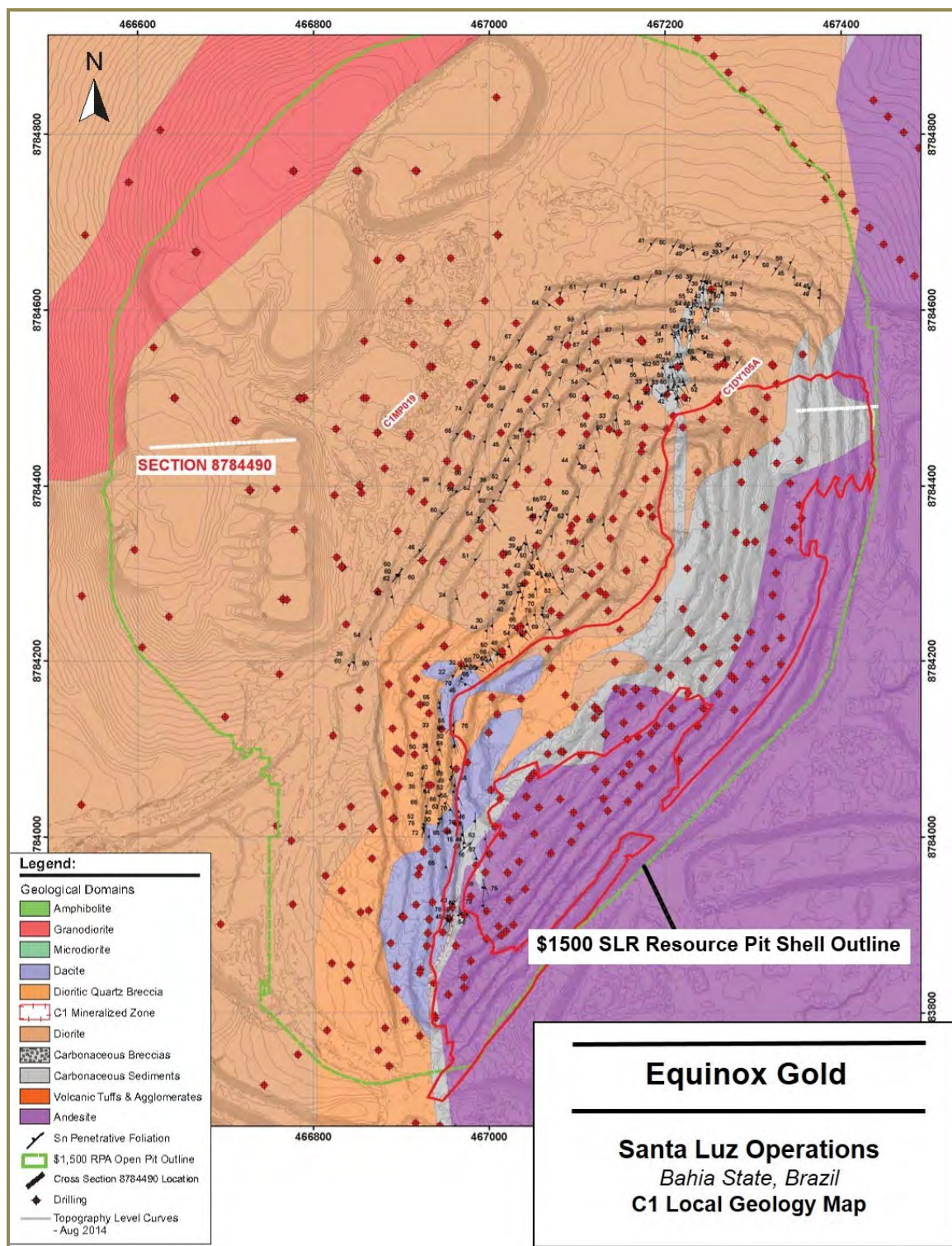
Figure 7-3: Santa Luz C1 Local Geology
