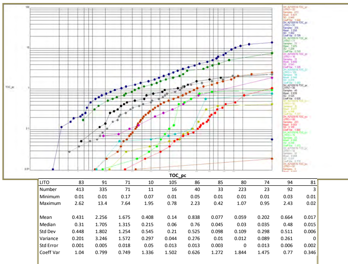
Figure 14-12: Antas 2 TOC Probability Plot by Lithology
