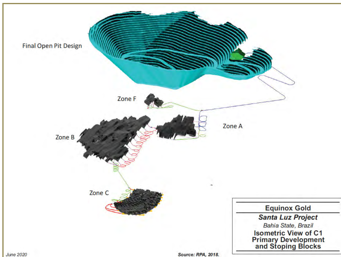
Figure 24-4: Isometric View of C1 Underground Primary Development and Stopping Blocks
