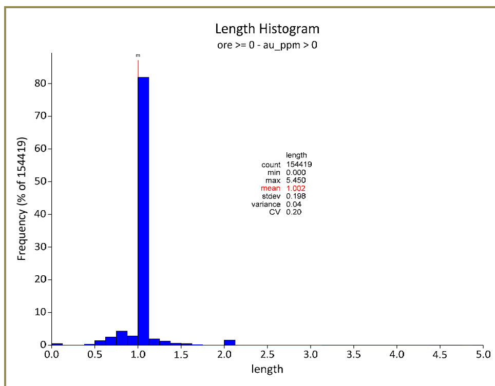
Figure 14-17: Histogram of Sample Lengths
