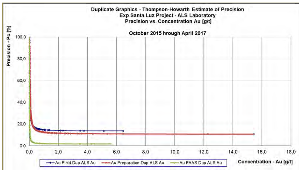
Figure 11-6: Thompson Howarth Criteria—Duplicates Performance for Gold (2015–2017)
