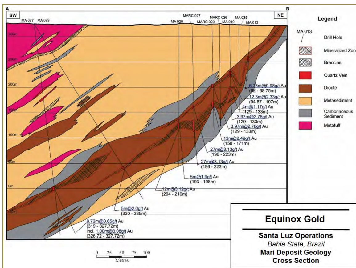
Figure 7-9: Mari Deposit Geologic Cross Section
