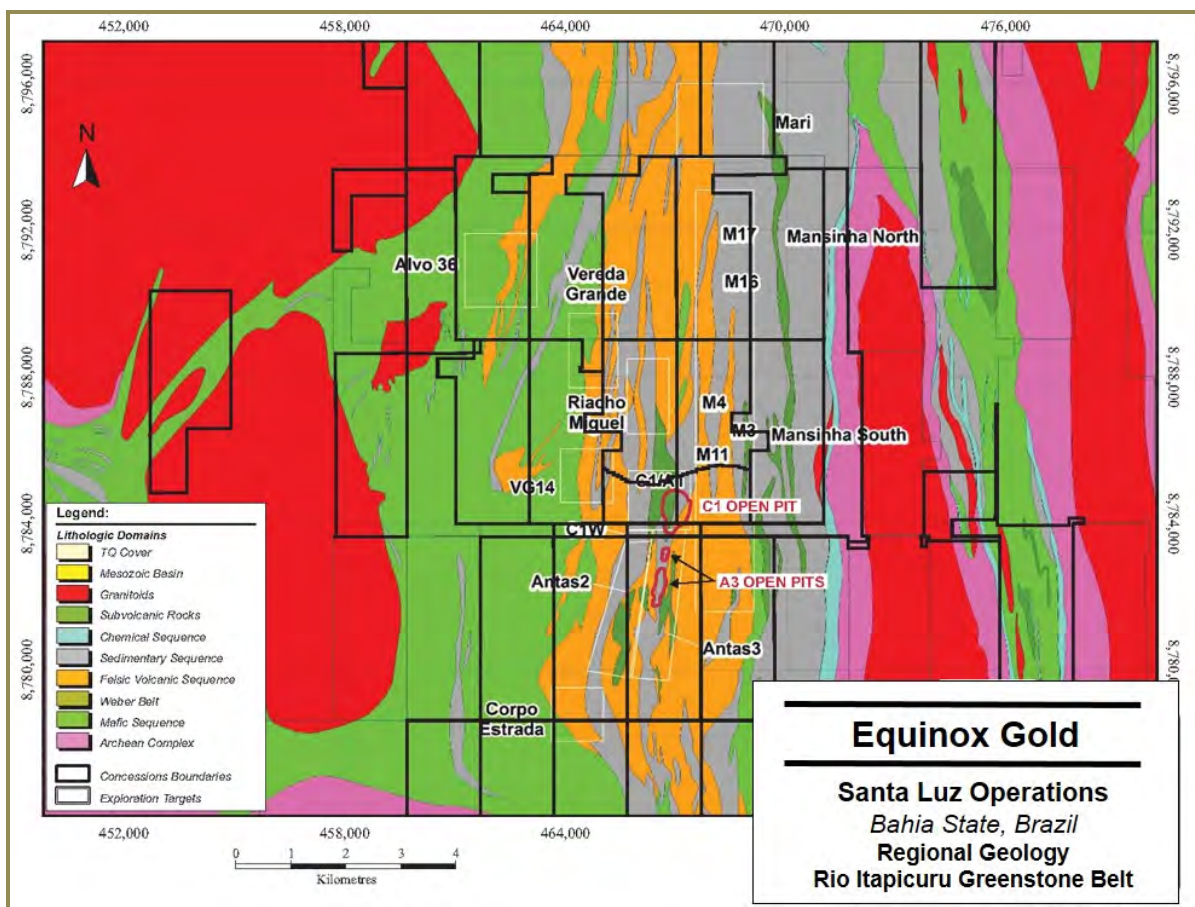
Figure 7-1: Regional Geology—Rio Itapicuru Greenstone Belt
