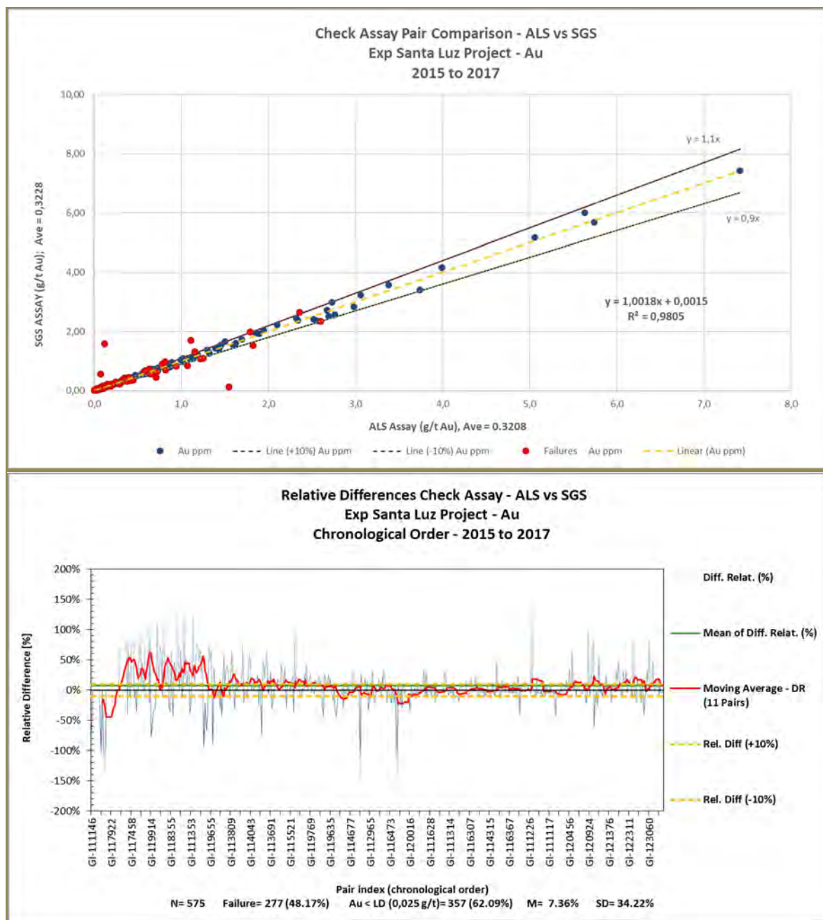
Figure 11-7: Comparison and Chronological Order for Check Assay Results (2015–2017)
