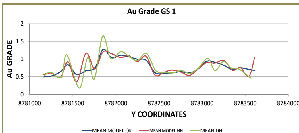
Figure 14-29: Drift Analysis of Antas 3 Grade Shell Block Estimates vs. NN Composite
