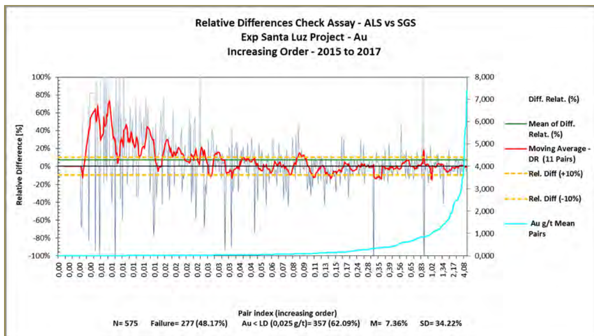
Figure 11-8: Increasing Order for Check Assay Results (2015–2017)
