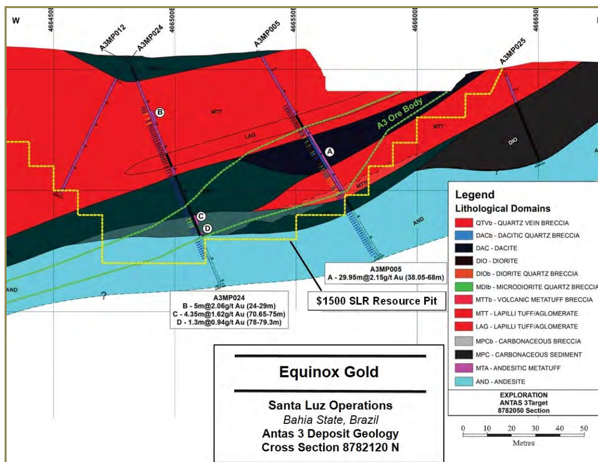
Figure 7-6: Antas 3 Deposit Geologic Cross Section 878 2120
