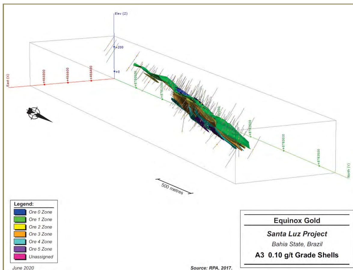
Figure 14-10: Antas 3 0.10 g/t Grade Shells
