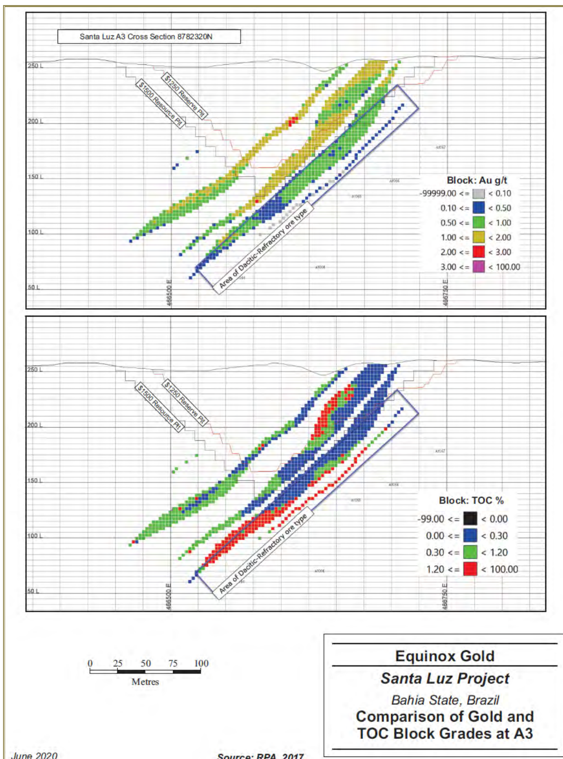
Figure 14-27: Comparison of Gold and TOC Block Grades at Antas 3
