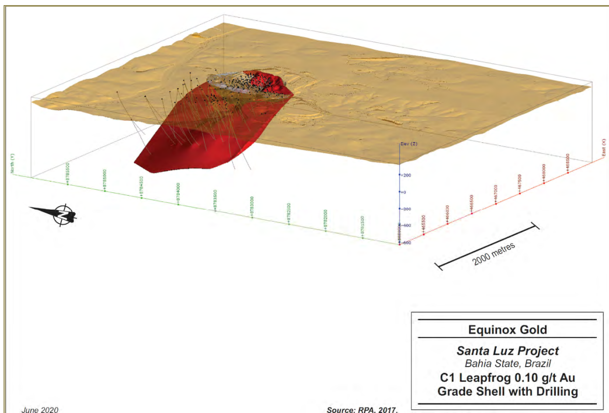
Figure 14-3: C1 Leapfrog 0.10 g/t Au Grade Shell with Drilling
