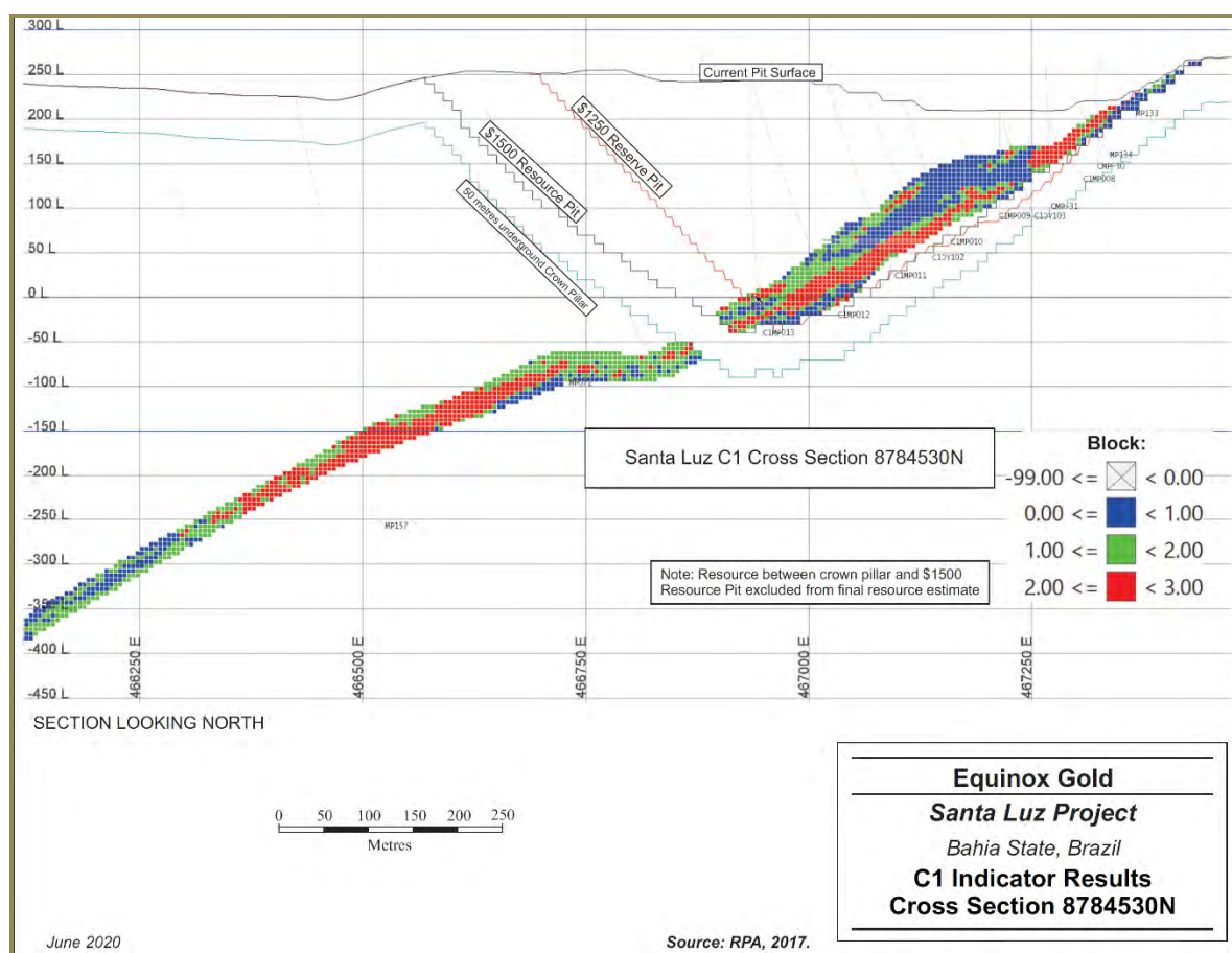
Figure 14-6: C1 Indicator Results Cross Section 8784530N
