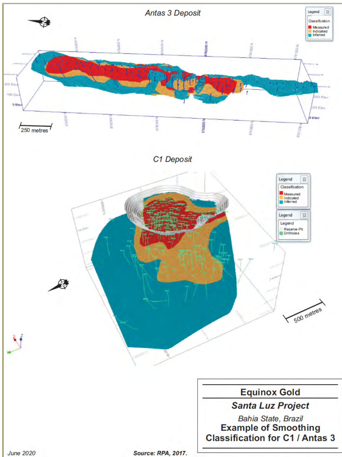
Figure 14-32: Example of Smoothing Classification for C1 and Antas 3
