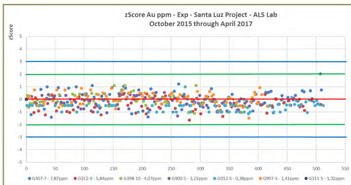
Figure 11-1: Score Chart of Au CRM Results (2015–2017)
