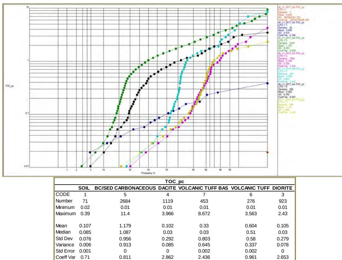
Figure 14-11: C1 TOC Probability Plot by Lithology
