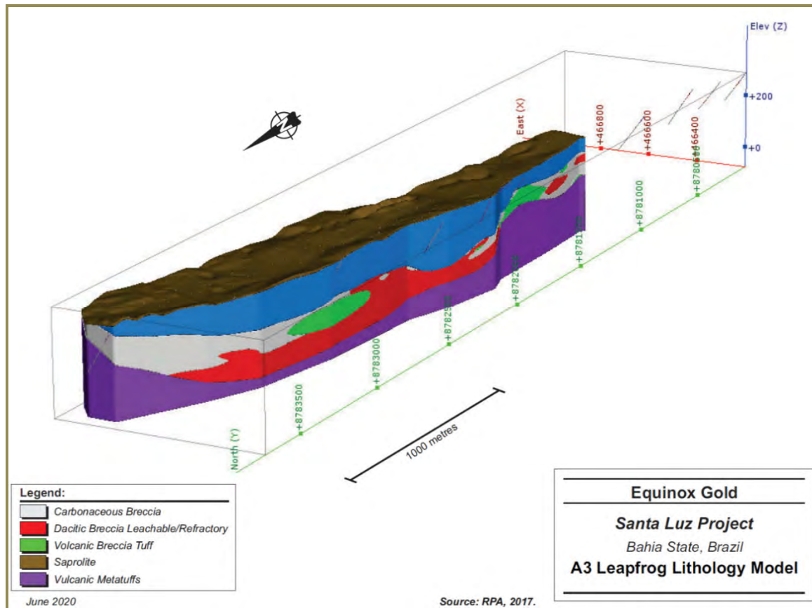
Figure 14-9: Antas 3 Leapfrog Lithology Model
