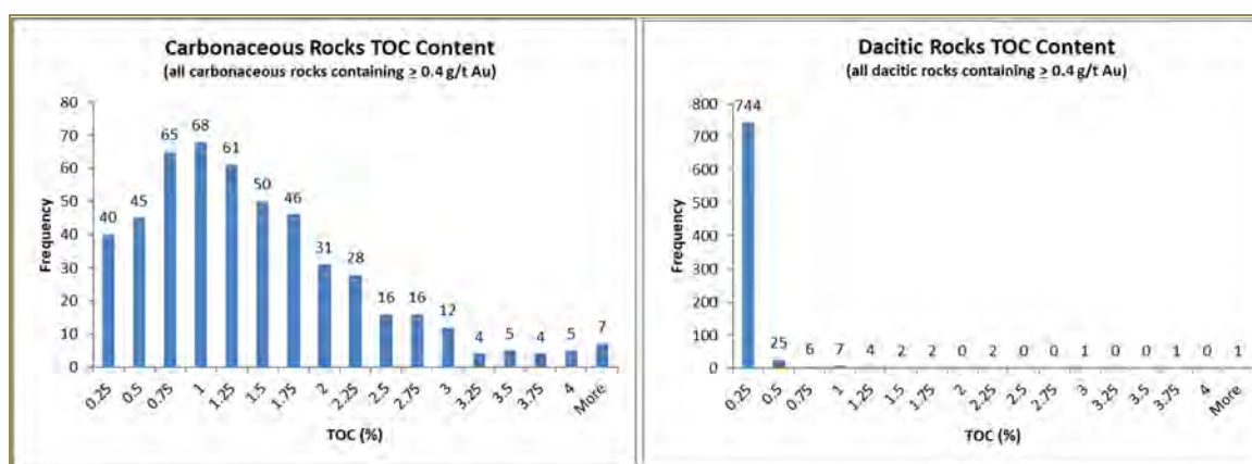
Figure 7-7: Carbonaceous and Dacitic Rocks TOC Contents
