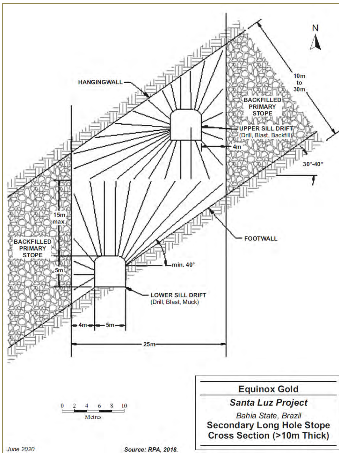
Figure 24-7: Secondary Long Hole Stope Cross Section (>10 m Thick)
