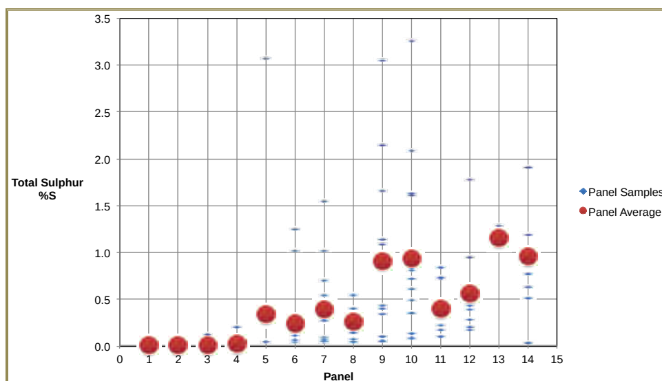
Figure 20-1: Mine Panel Sulphur Grade
