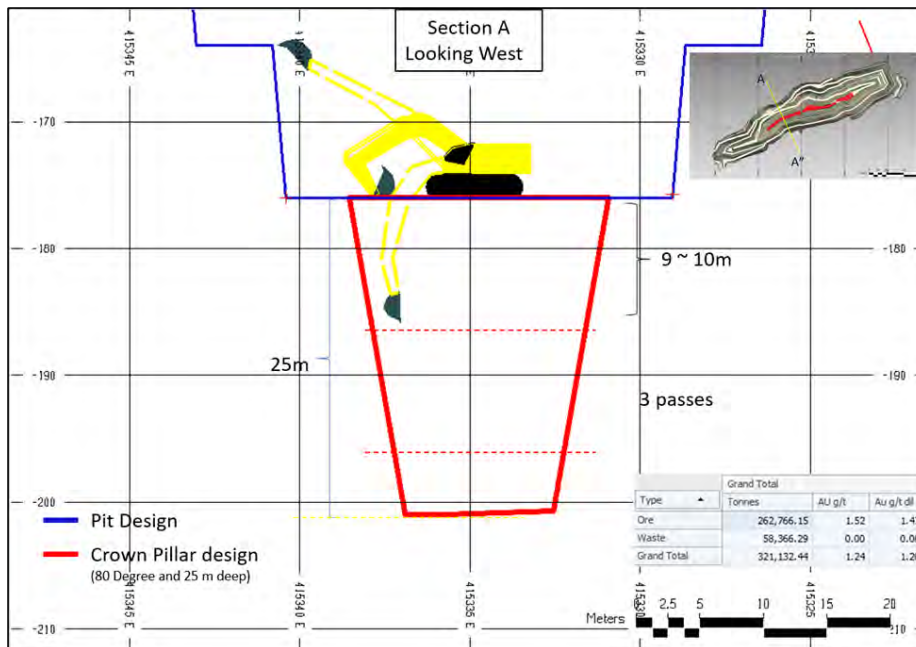
Figure 16-29: Crown Pillar – Area A Design
