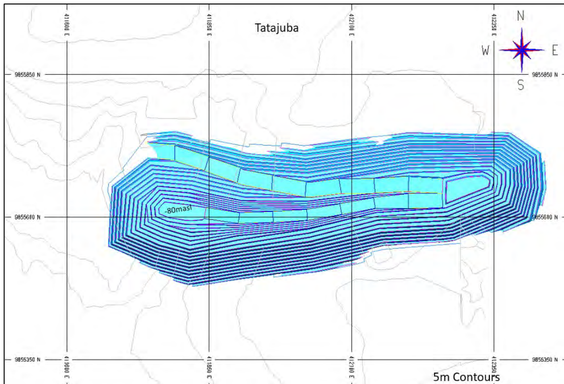
Figure 16-25: Tatajuba Pit Design – Phase 2
