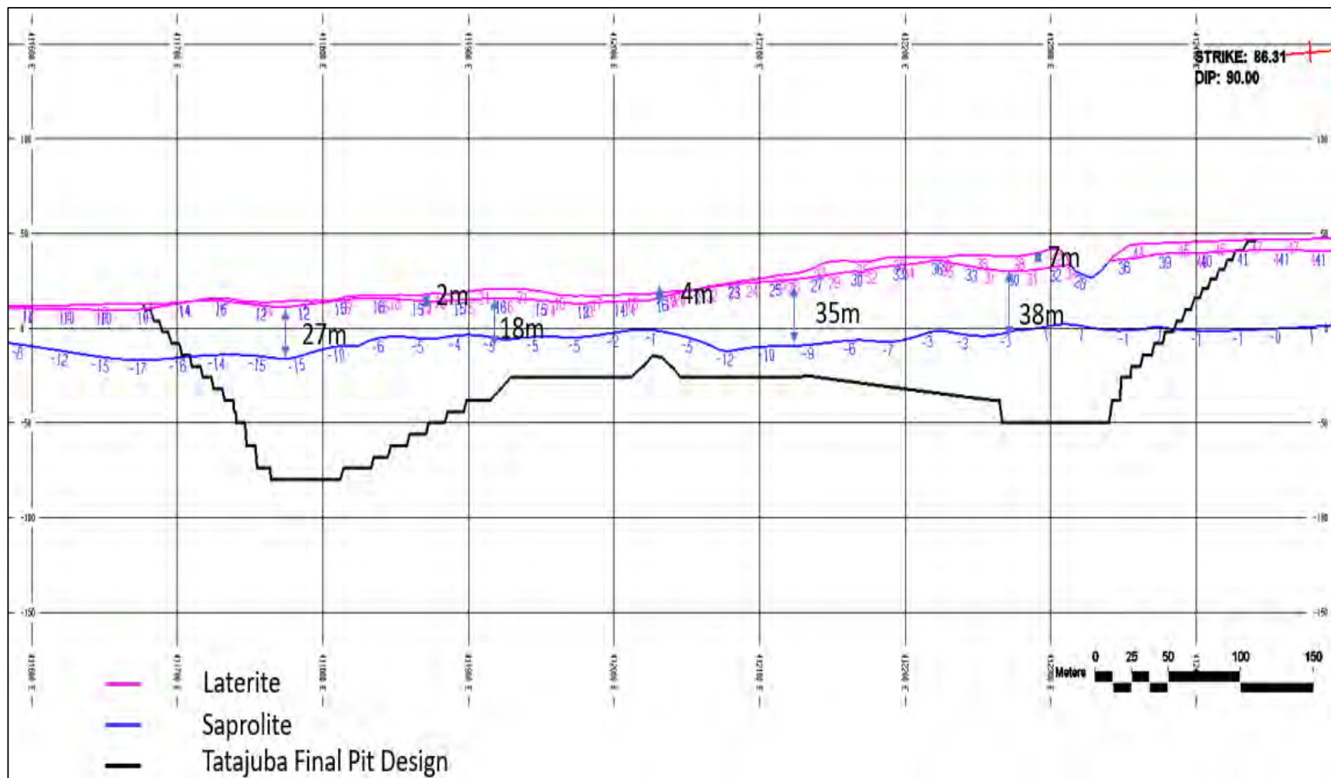
Figure 16-6: Tatajuba – Longitudinal Cross-section looking South
