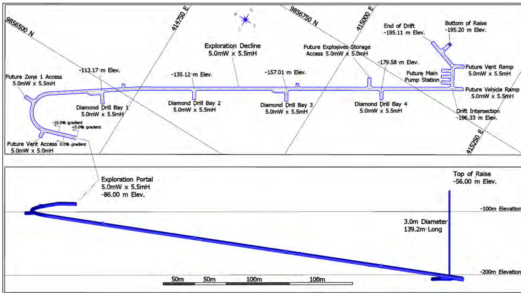
Figure 16-35: Exploration Decline Layout
