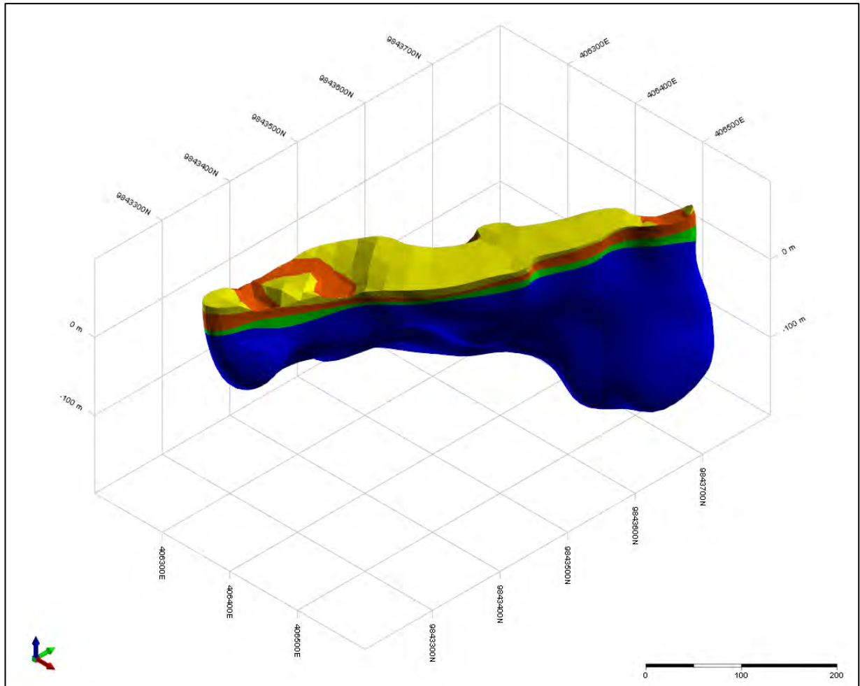
Figure 14-42: Isometric View of Touro Mineralization Model
