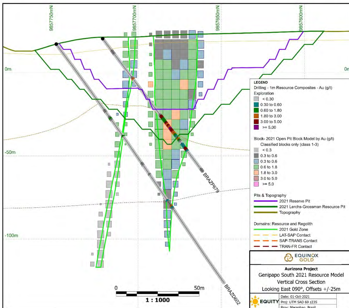
Figure 14-39: Cross Section of the Genipapo South Open Pit Block Model
