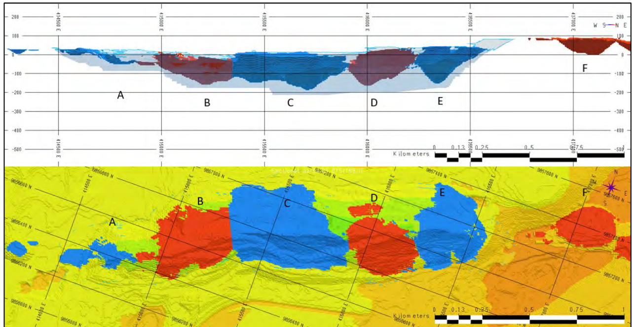
Figure 16-13: Piaba Pit Phase Analysis
