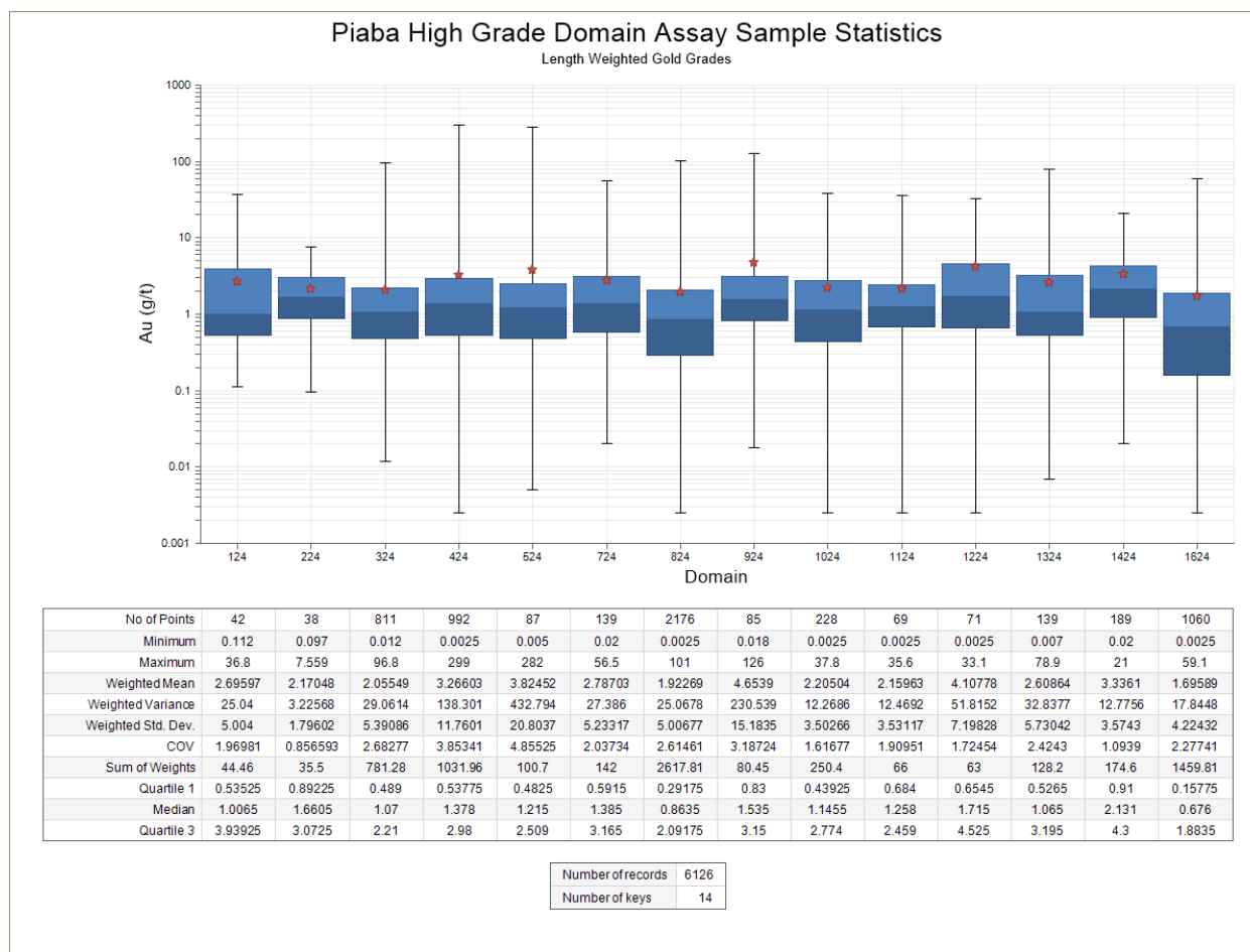
Figure 14-10: Boxplot of Piaba High-grade Domain Assay Sample Statistics
