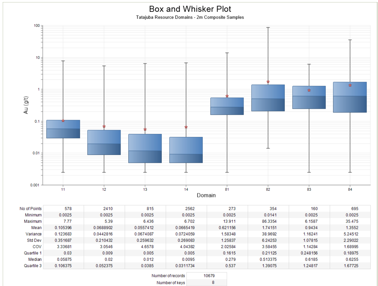
Figure 14-25: Boxplot of 2 m Composite Samples for Tatajuba Deposit Area
