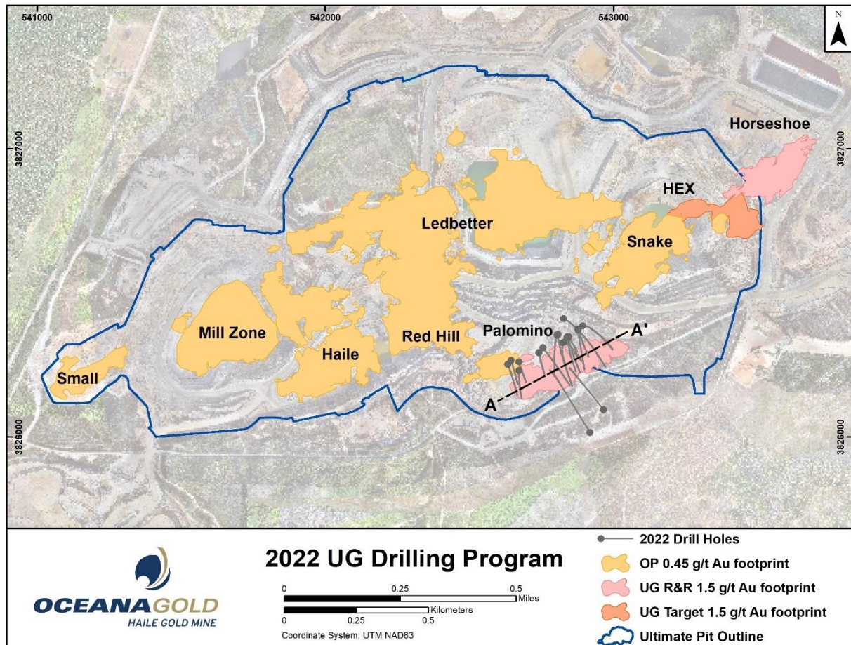
Figure 5: Plan view of the Haile Gold Mine with the reserve pit outline, open pit and underground mineralisation footprints and 2022 drill hole traces
