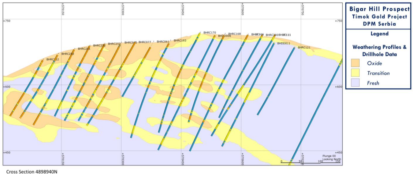
Figure 4. Cross section 4898940N through the Bigar Hill prospect showing the weathering profiles and drill hole interval data, assigned by review of five-metre composite bottle roll assays and geologic re-logging data. Looking North.
