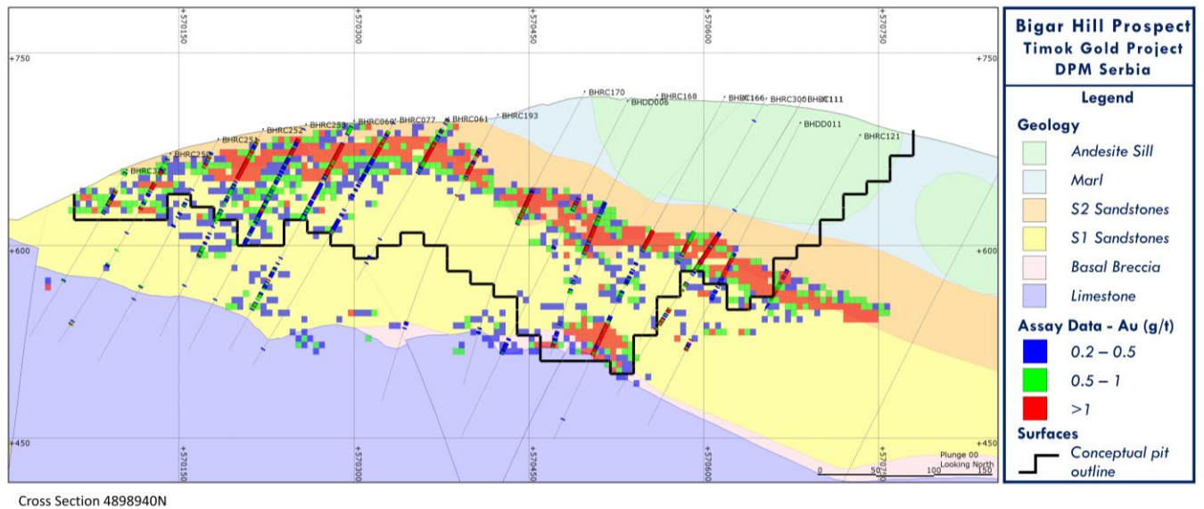
Figure 3 Cross section 4898940N through the Bigar Hill prospect showing the geologic model overlain by the block model, drill hole data and conceptual pit optimisation outline. Looking North.
