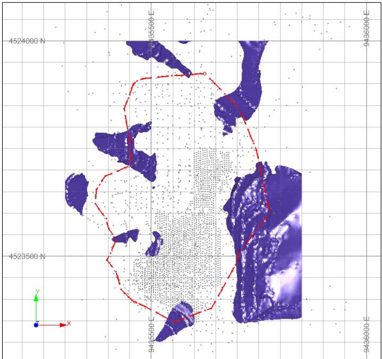
Figure 14-3: Overburden solids representing ancient mining spoils
