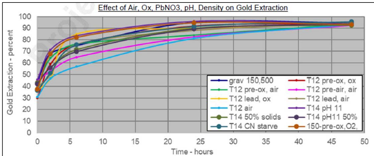
Figure 13-2 Effect of Various Parameters on Leaching Rate (source: BaseMet, 2019)
