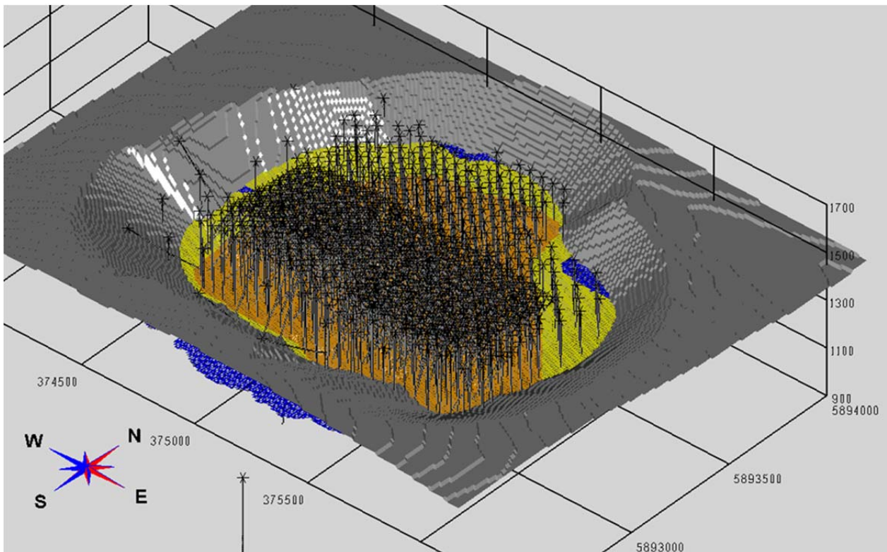
Figure 14-7 Three-dimensional View of the Classification at elev.=1350 (mid pit), the Drill Pattern, and the Resource Pit (source, MMTS, 2020)
