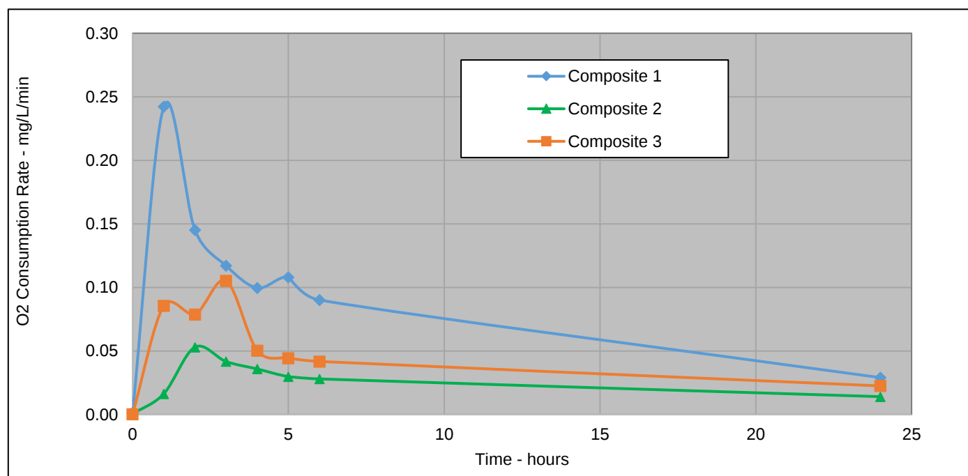
Figure 13-1: Oxygen Uptake Rate for the Three Composites
