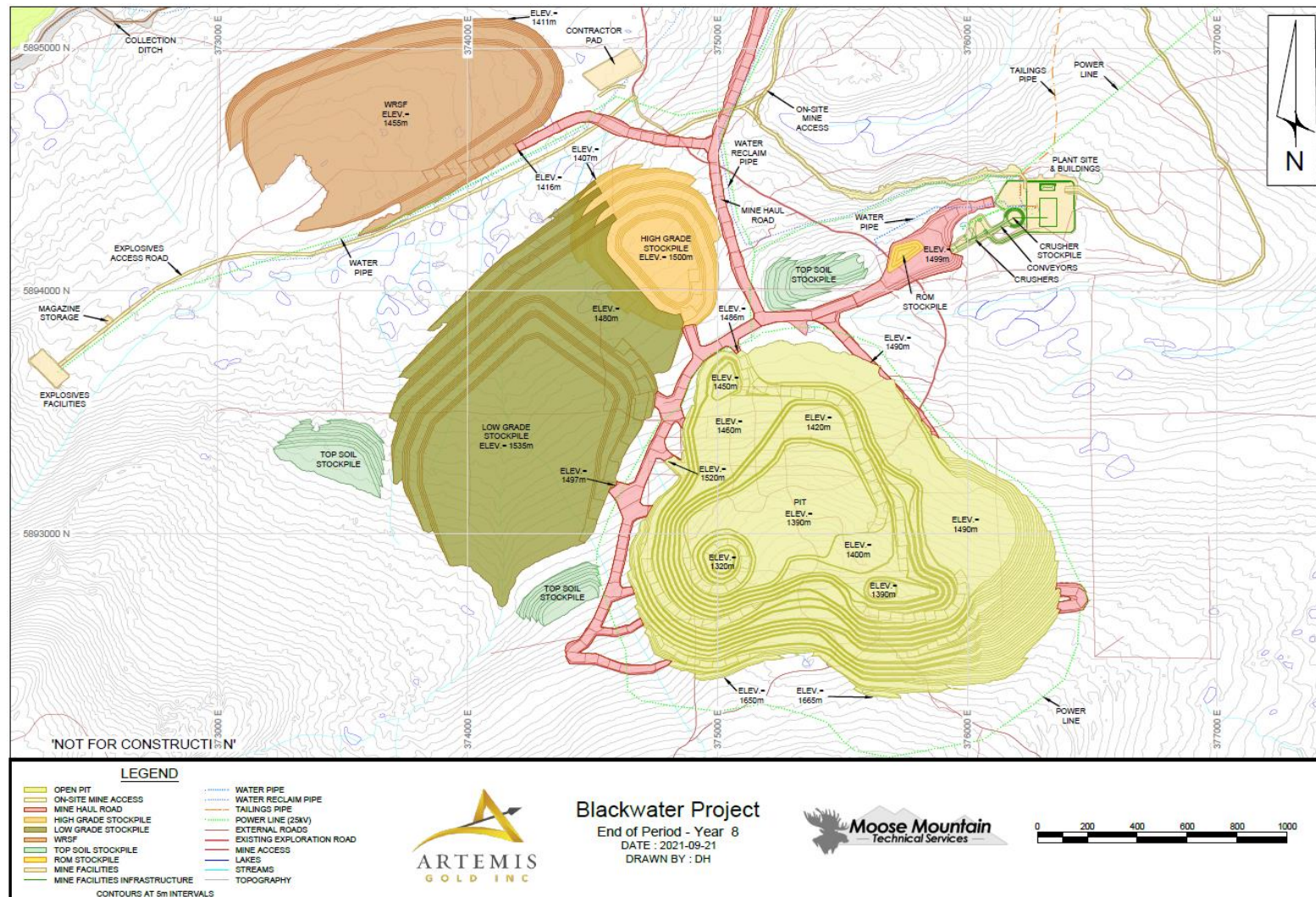
Figure 16-26: EOP Mine Operations, Y8
