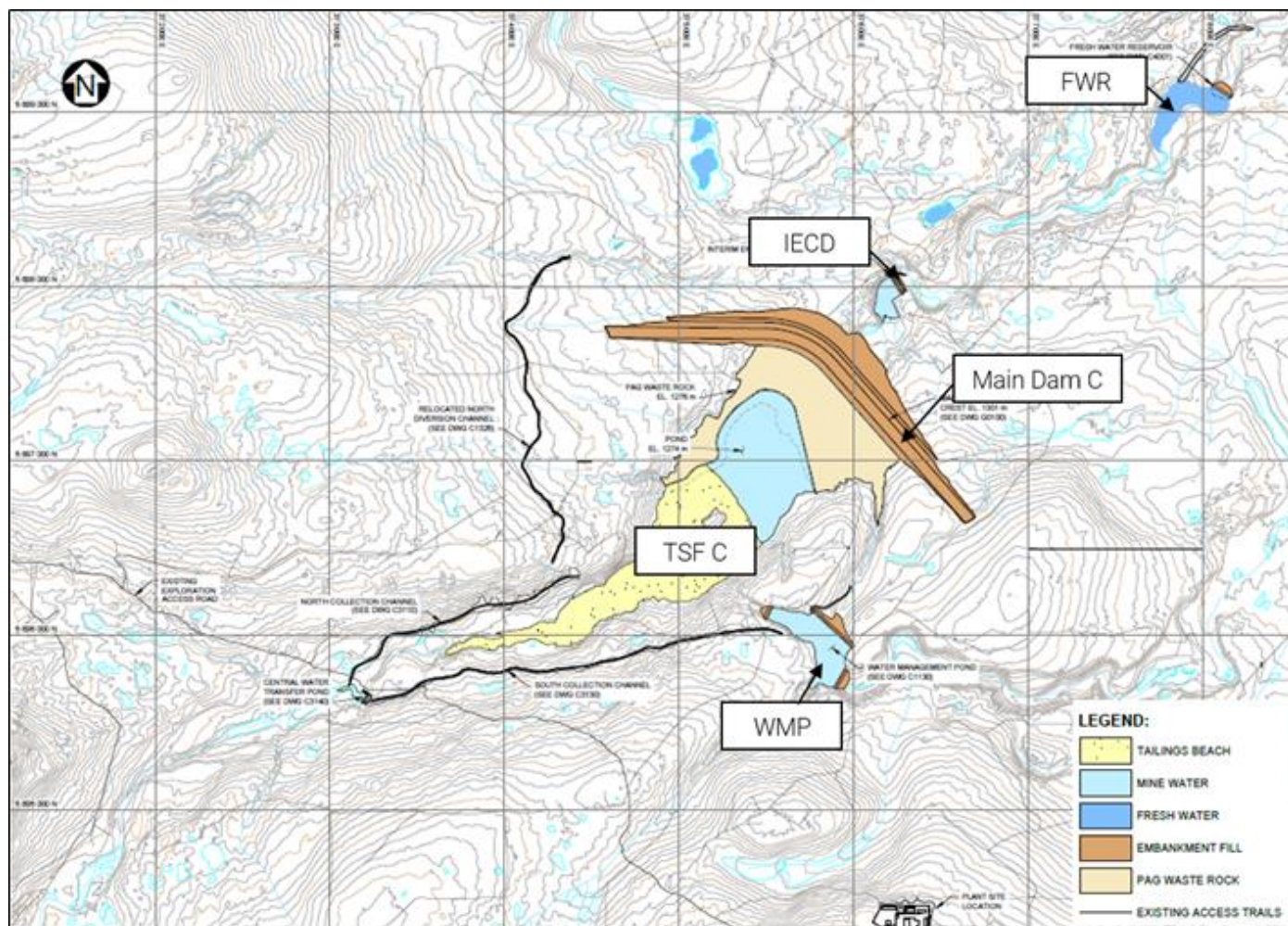
Figure 18-4: TSF General Arrangement – End of Year 3
