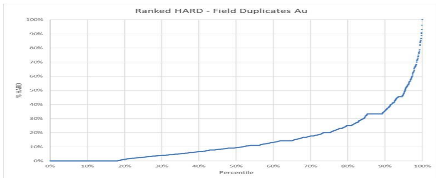
Figure 11-4: Field Duplicates Ranked HARD plot – Au
