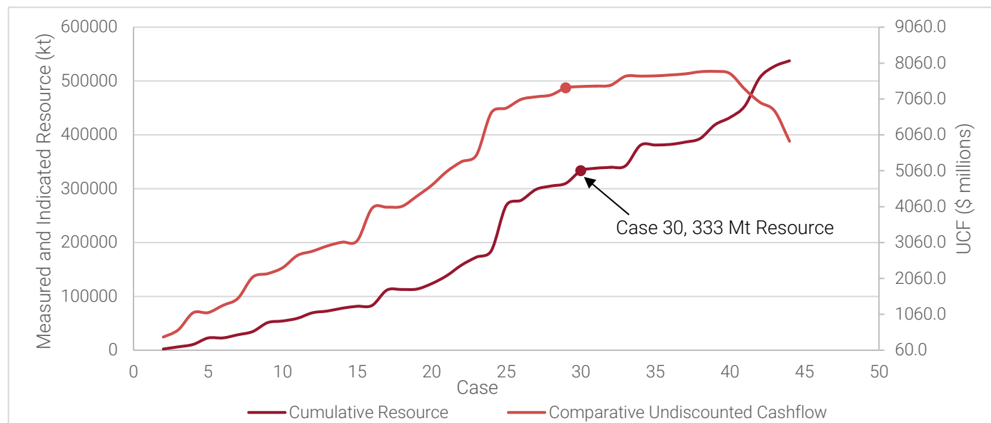
Figure 16-2: Pseudoflow Pit Shell Resource Contents by Case
