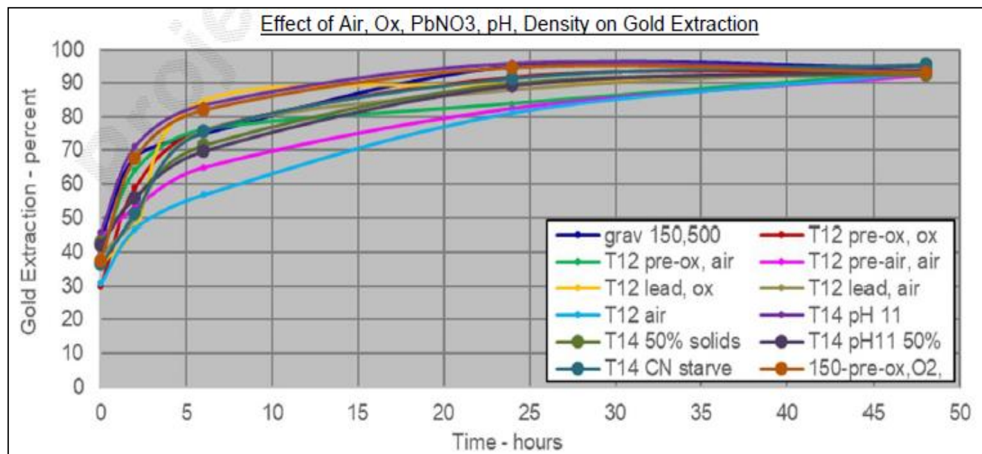
Figure 13-2: Effect of Various Leach Conditions on Gold Extraction
