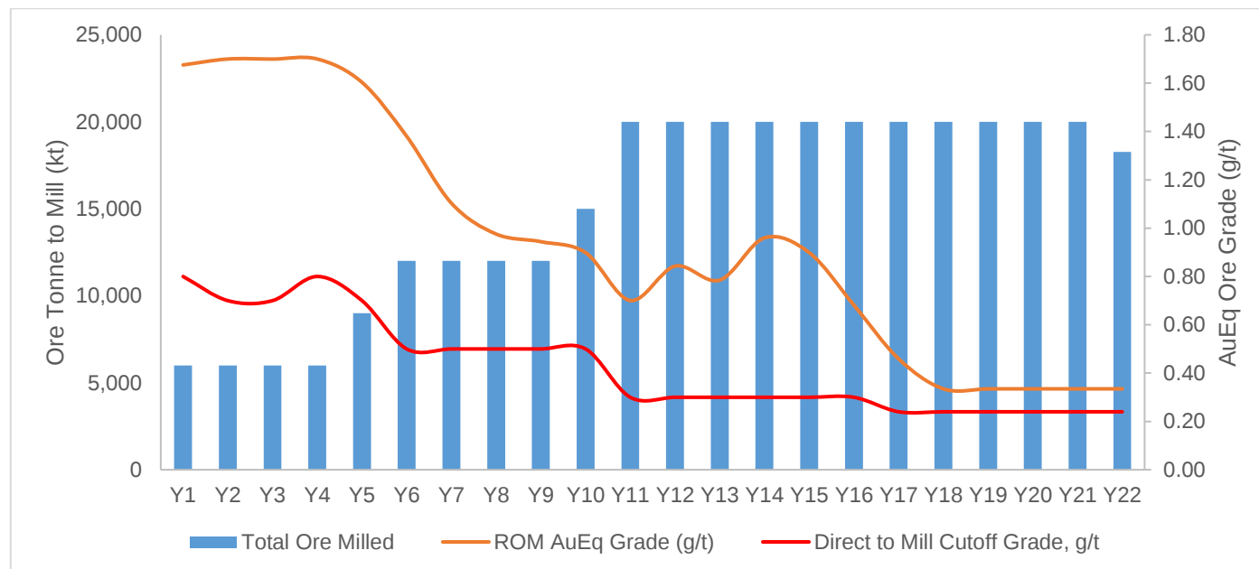
Figure 16-20: Planned Mill Feed Tonnes and Grade
