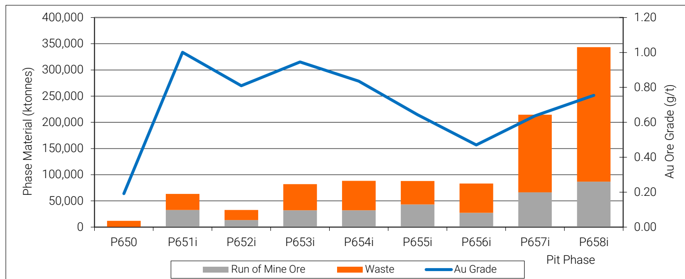
Figure 16-3: Designed Phase Pit Contents
