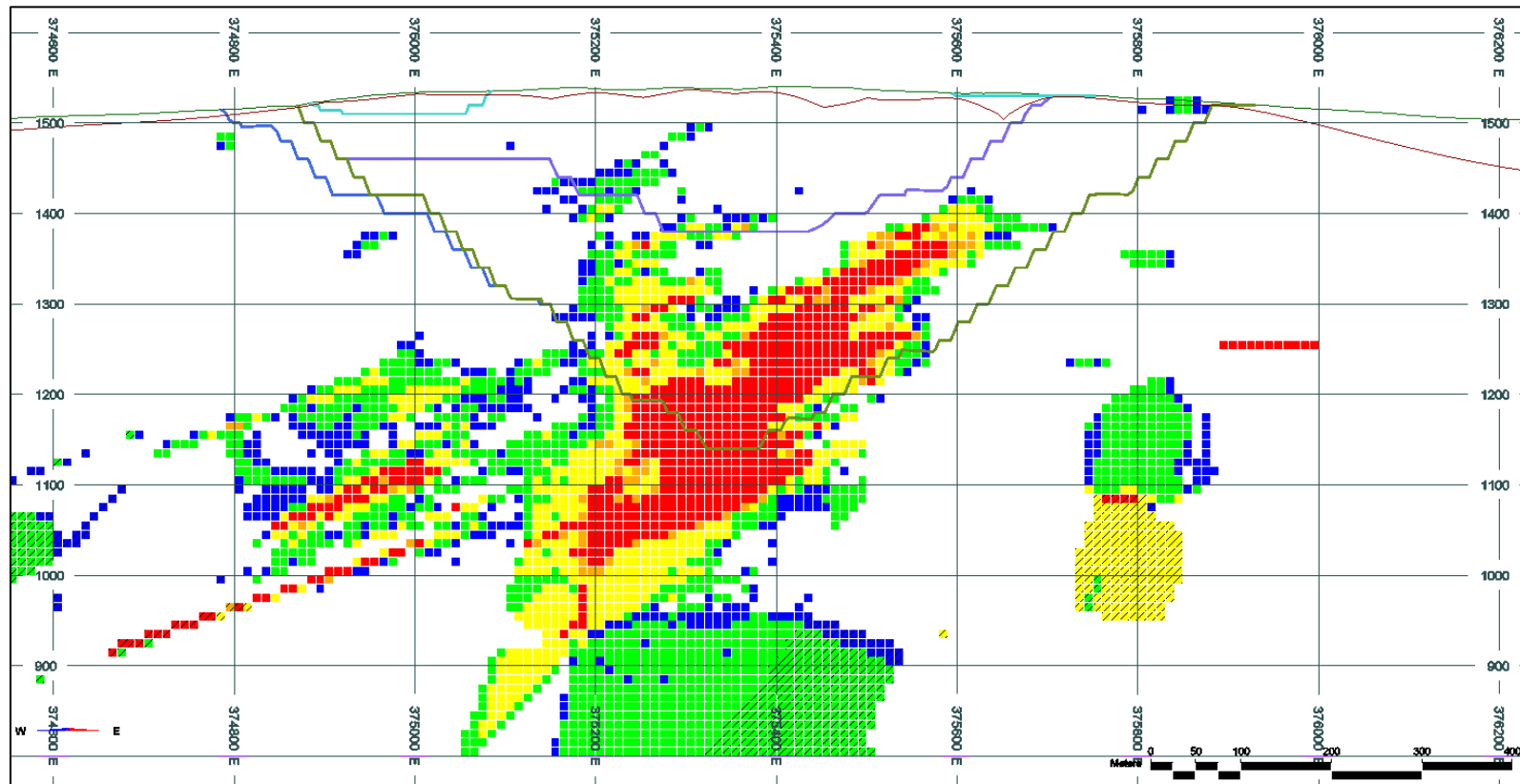
Figure 16-16: East West Section, 5,893,350N Looking North
