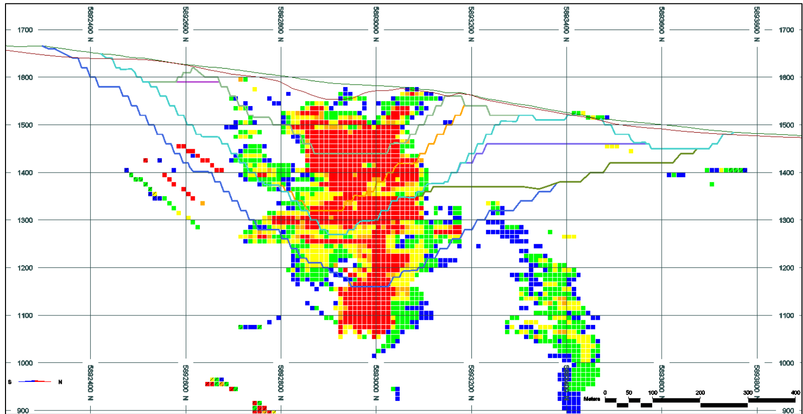
Figure 16-13: North South Section, 375,050E Looking West
