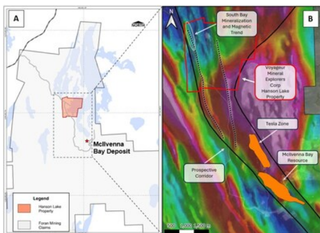
Figure 1 – A) Property map showing the Hanson Lake Property and its location relative to the McIlvenna Bay Deposit and adjacent Tesla Zone; B) Prospective corridor and magnetic trends from Foran 2023 Heli-TEM RMI merged with 2008 magnetic data from Copper Reef assessment reports on the Hanson Lake Property (CNW Group/Foran Mining Corporation)
