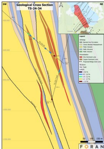
Figure 6 – Geological cross section through the Tesla Zone showing recently drilled TS-24-34 and the relationship between the Telsa Zone, the mineralization in the lower fault slice and the underlying Bridge Zone (CNW Group/Foran Mining Corporation)
