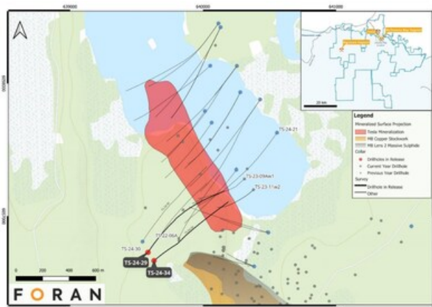
Figure 1 – Plan View of the Tesla Zone and Bridge Zone with location of drillholes TS-24-29 and TS-24-34 referred to in this news release, also showing the surface projections of interpreted Tesla and Mcllvanna Bay lenses (CNW Group/Foran Mining Corporation)
