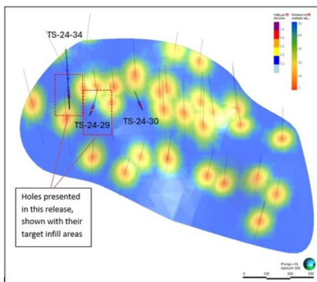
Figure 2 – Drilling density of the Tesla Zone displayed as coloured pierce points on a plane that represents the main lens of Tesla massive sulphide, with the hole traces for TS-24-29, -34 and also TS-24-30 (see the Company's October 7, 2024 news release) shown in black. Areas shown in blue are greater than 50m from the nearest drill hole intersection and correspond to target areas for infill drilling (CNW Group/Foran Mining Corporation)
