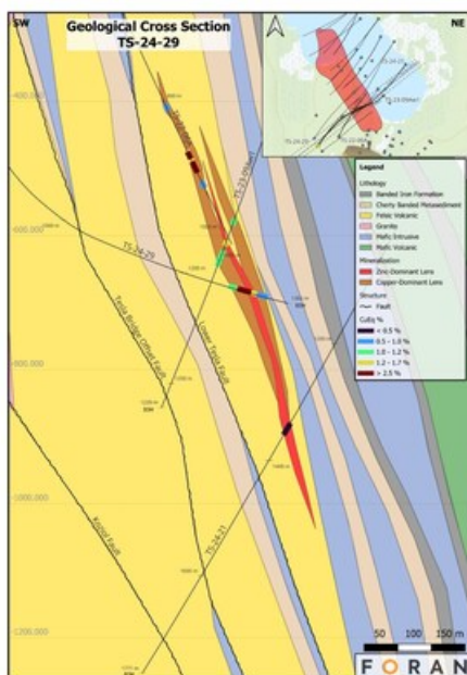
Figure 4 – Geological cross section through the Tesla Zone, highlighting the copper-dominant mineralization intersected in TS-24-29 (CNW Group/Foran Mining Corporation)
