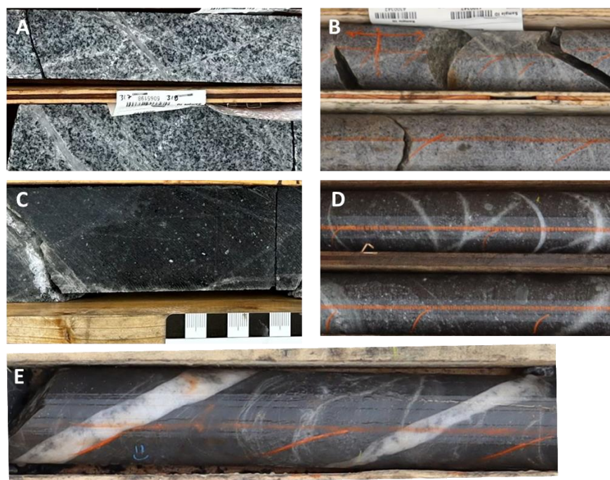
Figure 7-7: Lithological Units Defined from Valley Target Drillholes
