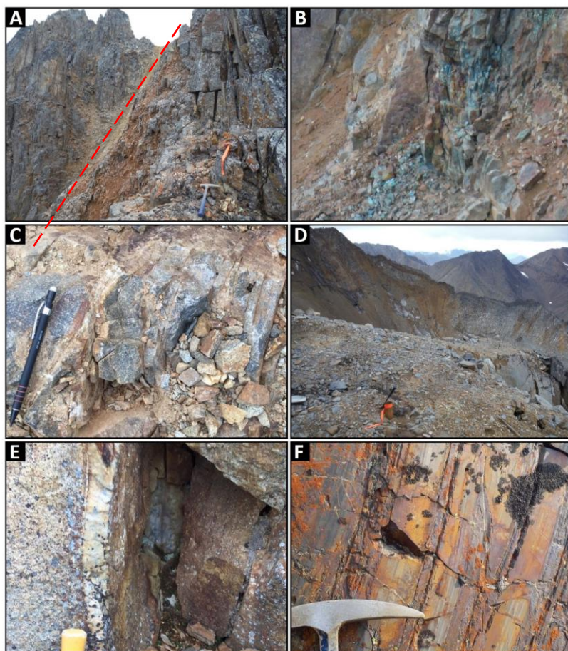
Figure 7-10: Orientation of Faults and Veins
