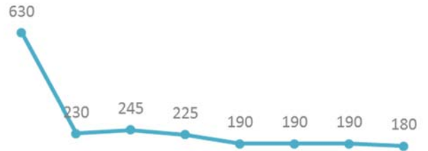
Indium
