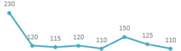
Gallium
