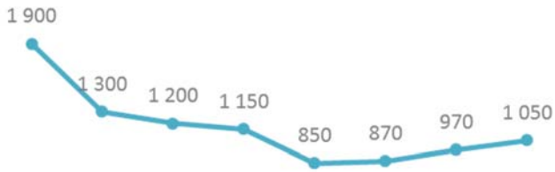
Germanium
