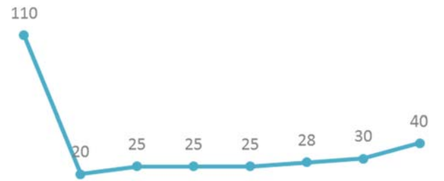
Tellure
