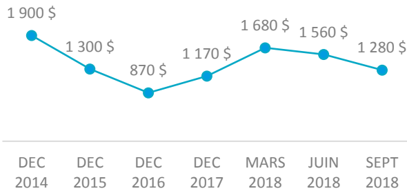
Germanium
