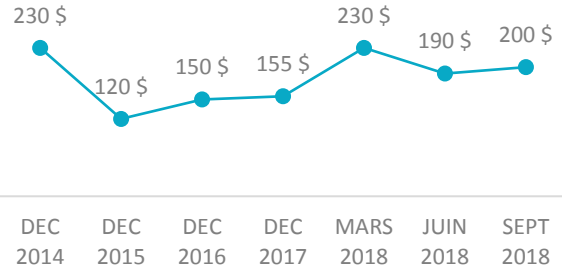
Gallium
