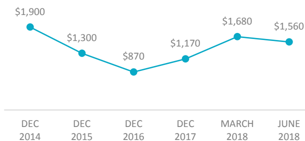
Germanium
