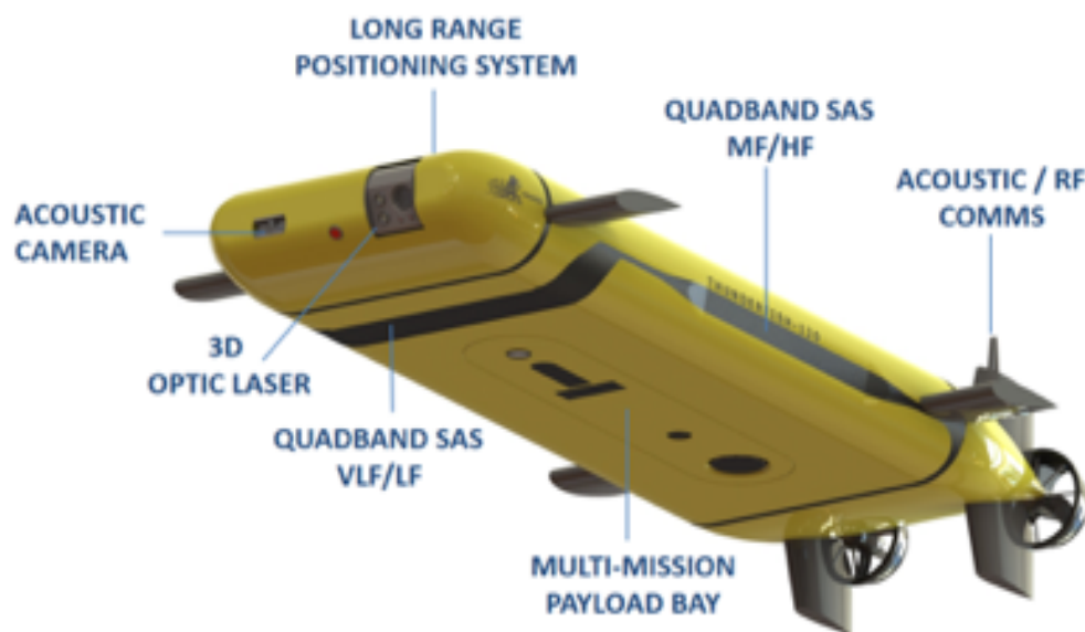
Figure 10: Multi-Spectral SAS on ThunderFish®
