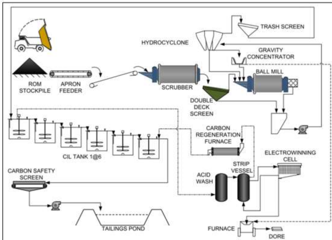
Figure 17-1 Current process flowsheet – Nampala mine
