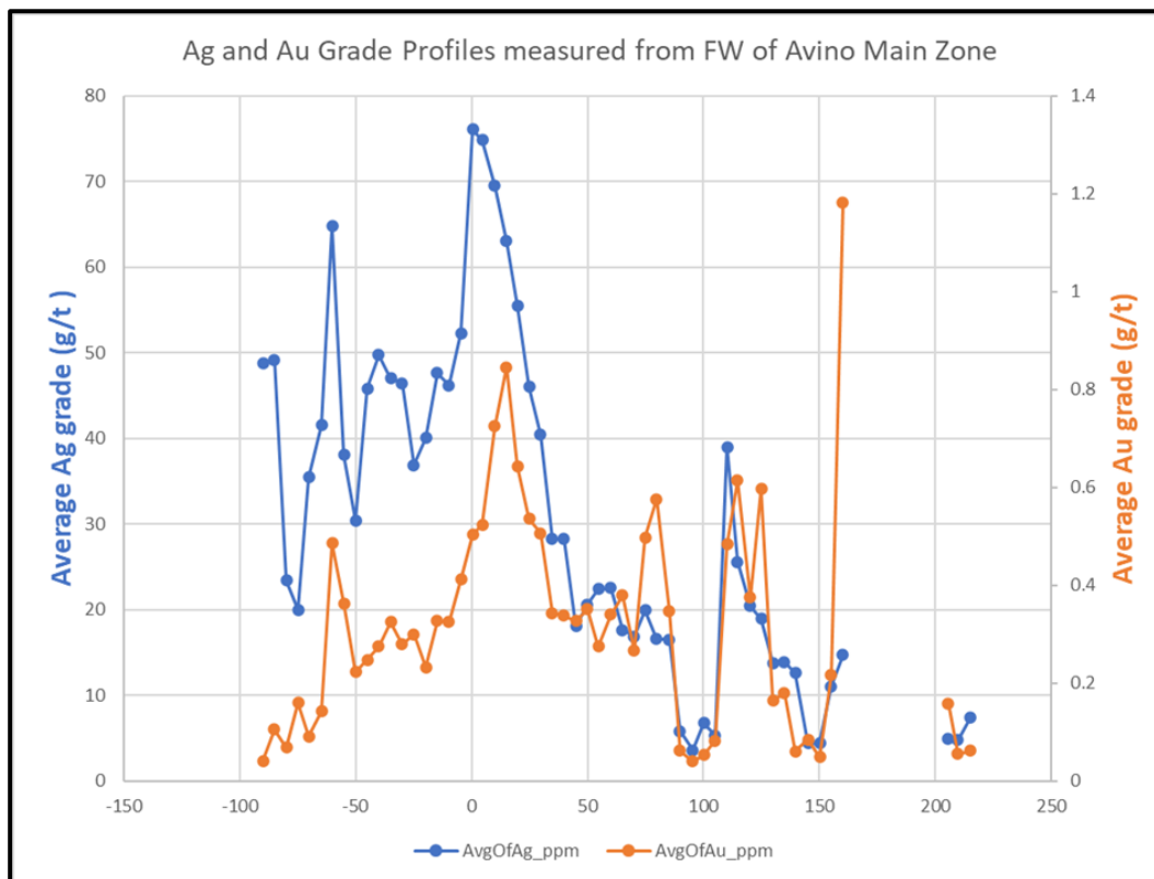
Figure 14.5 Silver and Gold Grade Profiles Relative the Avino Vein Main Zone Footwall
