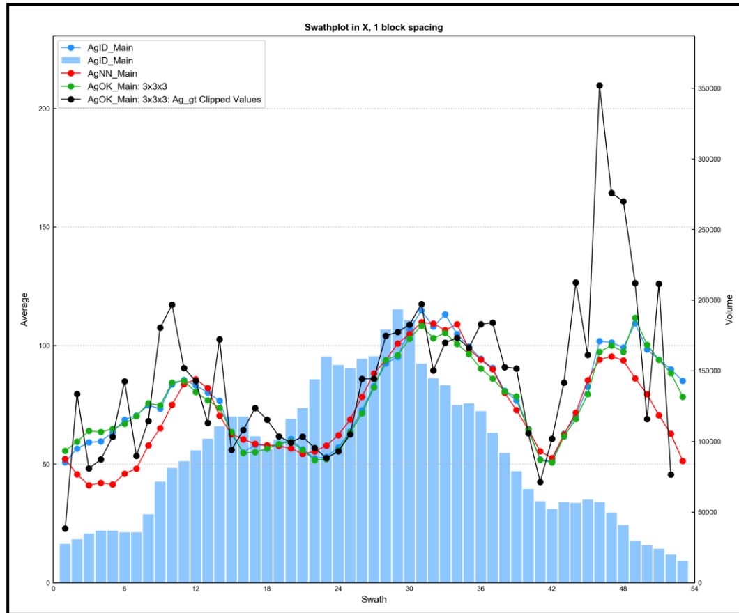
Figure 14.32 Avino Vein, Swath Plot for Silver, Eastings
