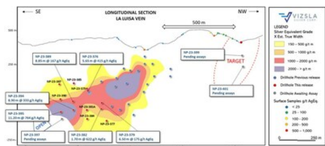
Figure 2: Longitudinal section of the La Luisa Vein. (CNW Group/Vizsla Silver Corp.)
