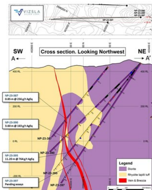
Figure 3: Cross section highlighting recent drill intercepts on La Luisa vein. (CNW Group/Vizsla Silver Corp.)
