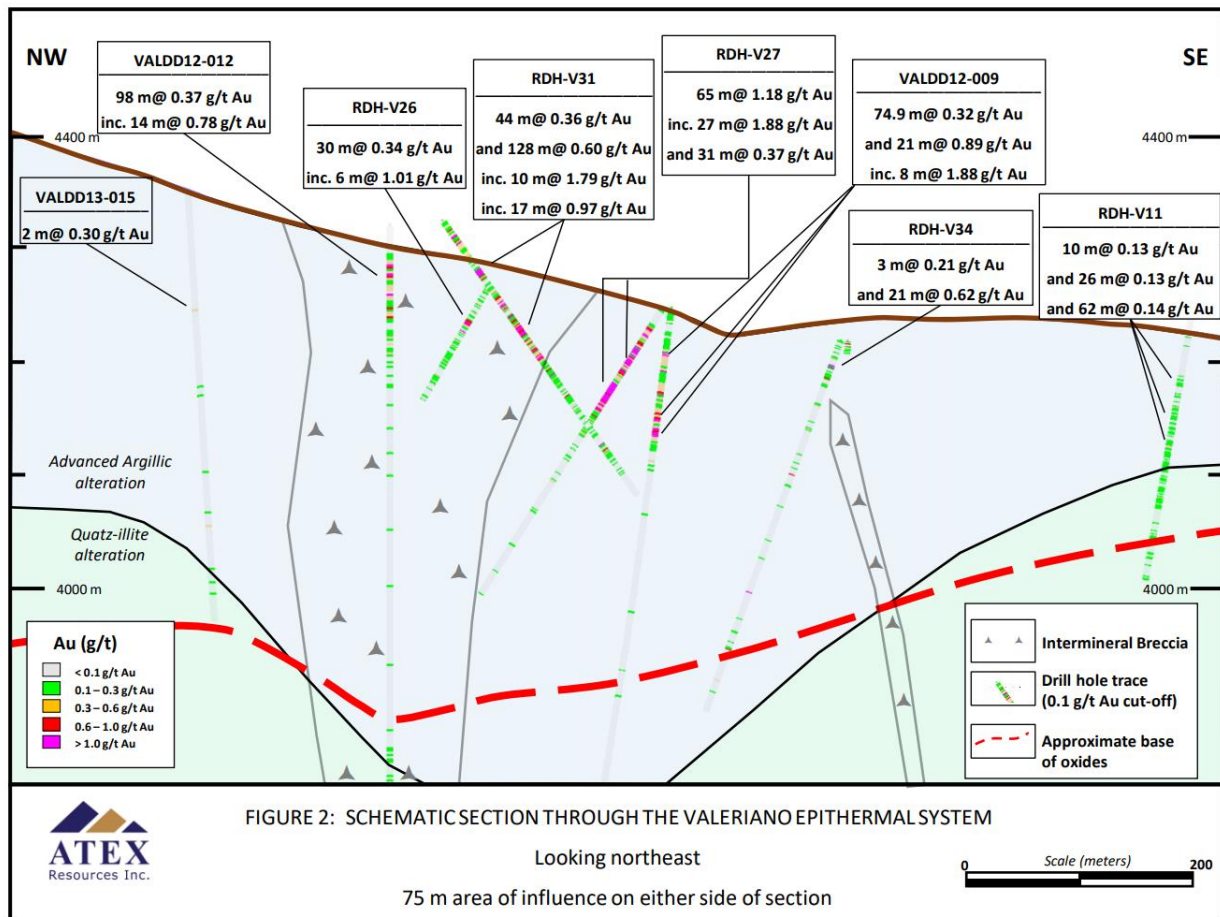
Figure 2. NW-SE section looking NE through the Central Zone. 75 m of influence on either side. The approximate base of oxidation is represented by the red dashed line. Within the gold mineralized envelope, to a depth of 230 m below surface, oxide mineralization occurs with mixed- and sulfide-mineralization. Assay intervals are based upon a 0.1 g/t Au cut off grade ("COG"). The COG used does not reflect any geological, economic or statistical control. Intercepts are defined on Au assay results only and make no consideration of geology. Up to 4 metres of internal dilution (samples below COG) were accepted. RDH refers to reverse circulation drill holes and DDH and VALDD refer to diamond drill holes.
