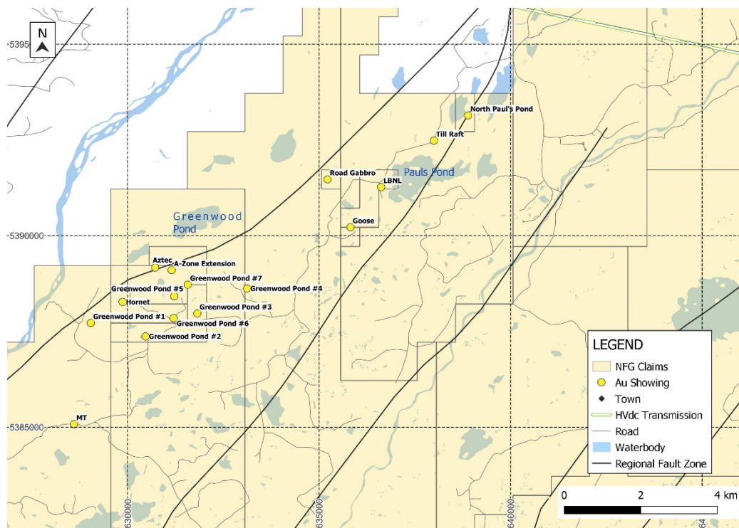
Queensway South Project – Locations of Gold Prospects
