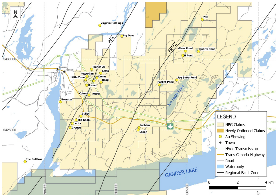
Queensway North Project – Locations of Gold Prospects along the AFZ and JBPfZ.
