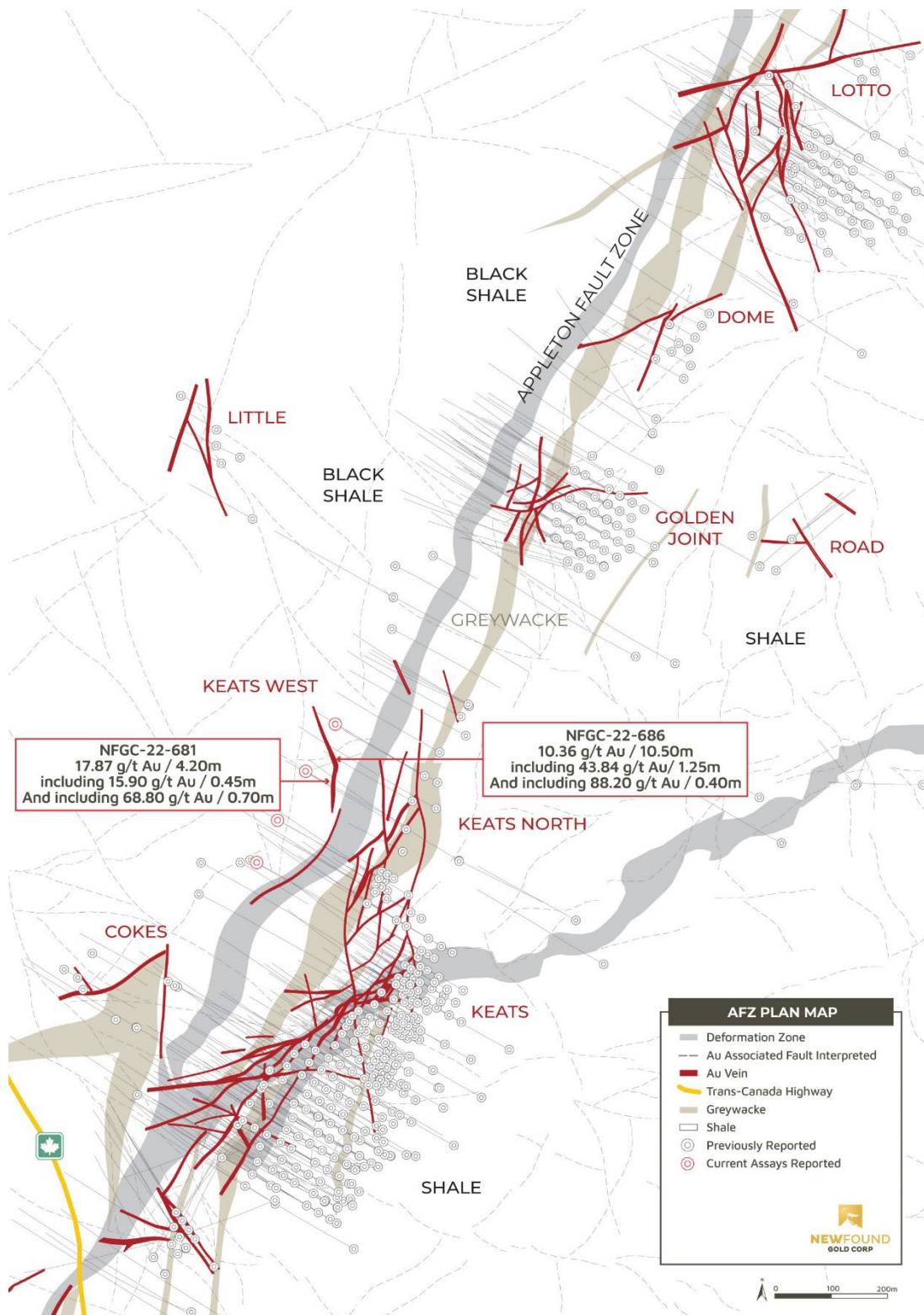
Queensway Project – Plan View Map of Keats – Lotto with Location of Keats West Discoveries (September 27, 2022)
