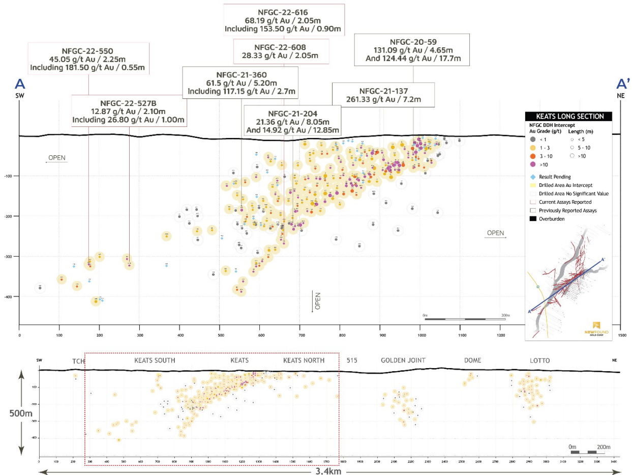
Queensway Project – Long Section of Keats Main Zone (October 18, 2022)
