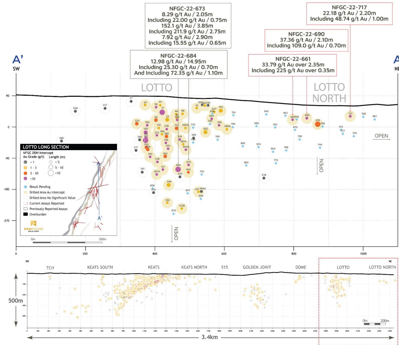
Queensway Project – Lotto- Lotto North Zones Long Section (November 2, 2022)
