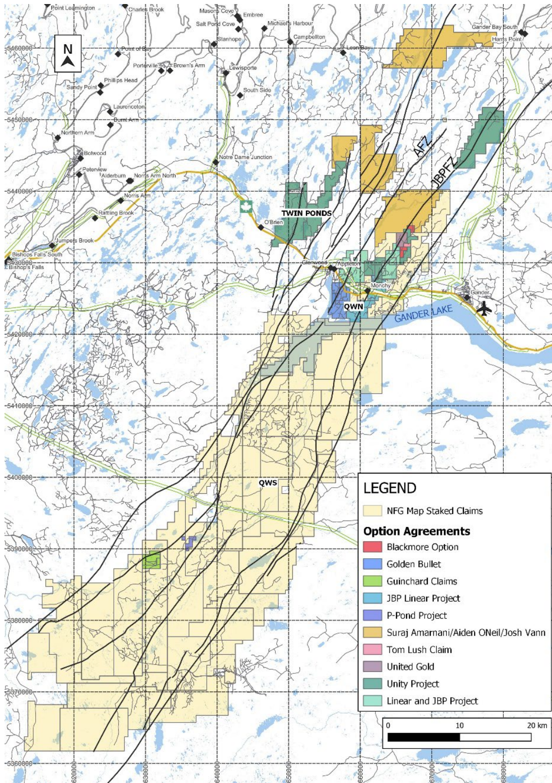
Queensway Project – Option Agreement Claim Groups
