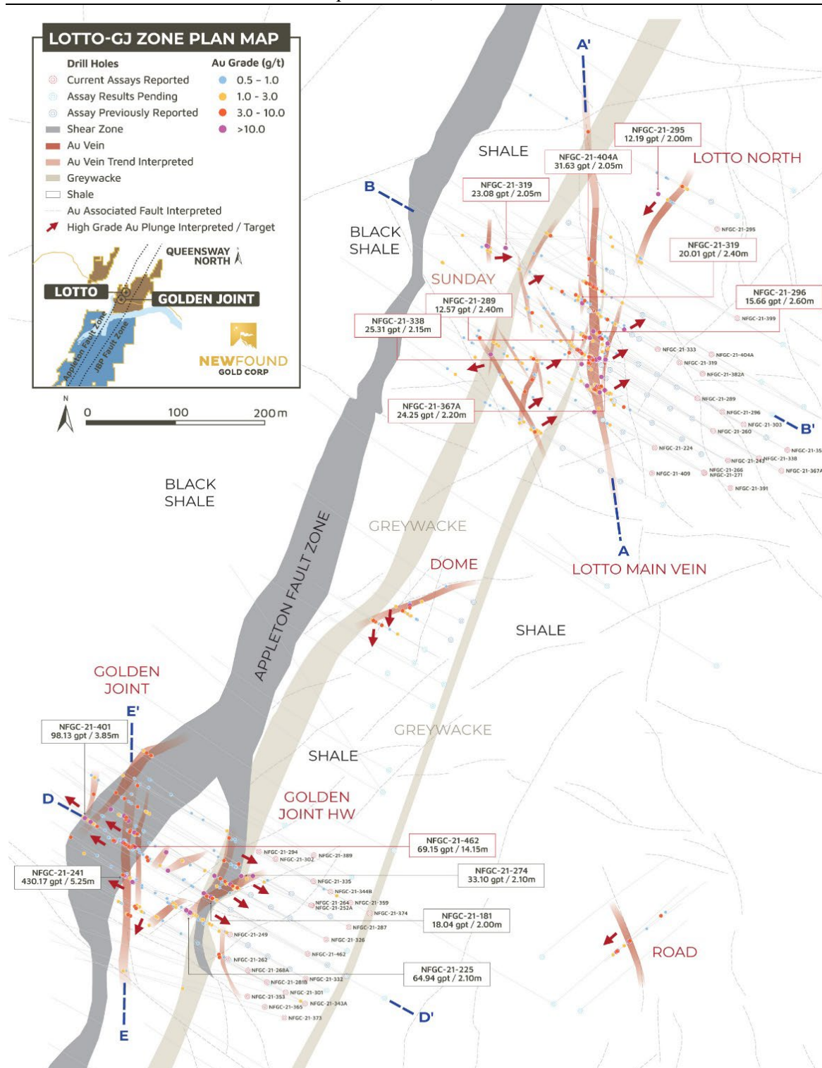
Queensway Project – Golden Joint – Lotto Zones Plan Map (March 24, 2022)
