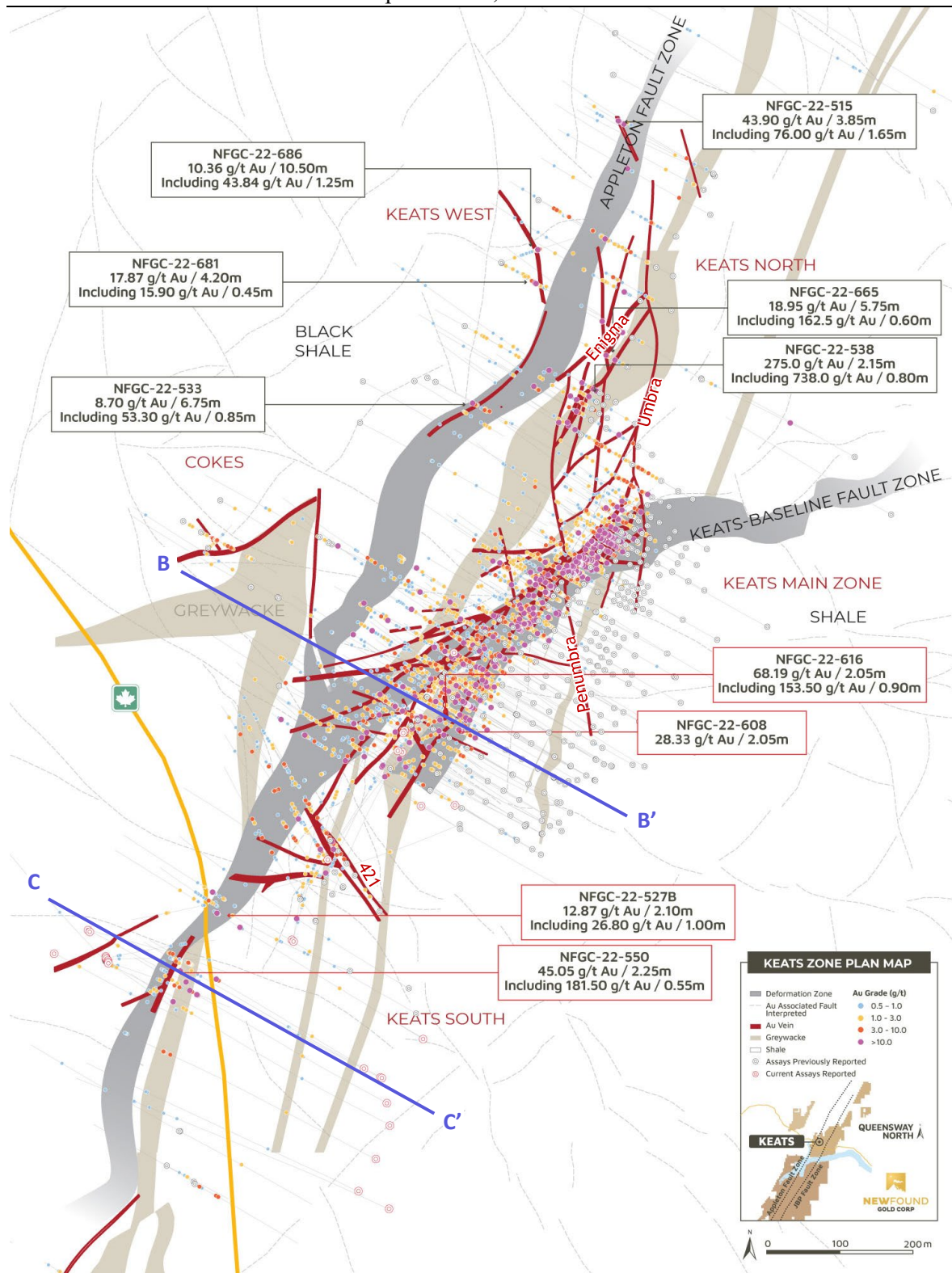
Queensway Project – Keats Plan View Map (October 18, 2022)
