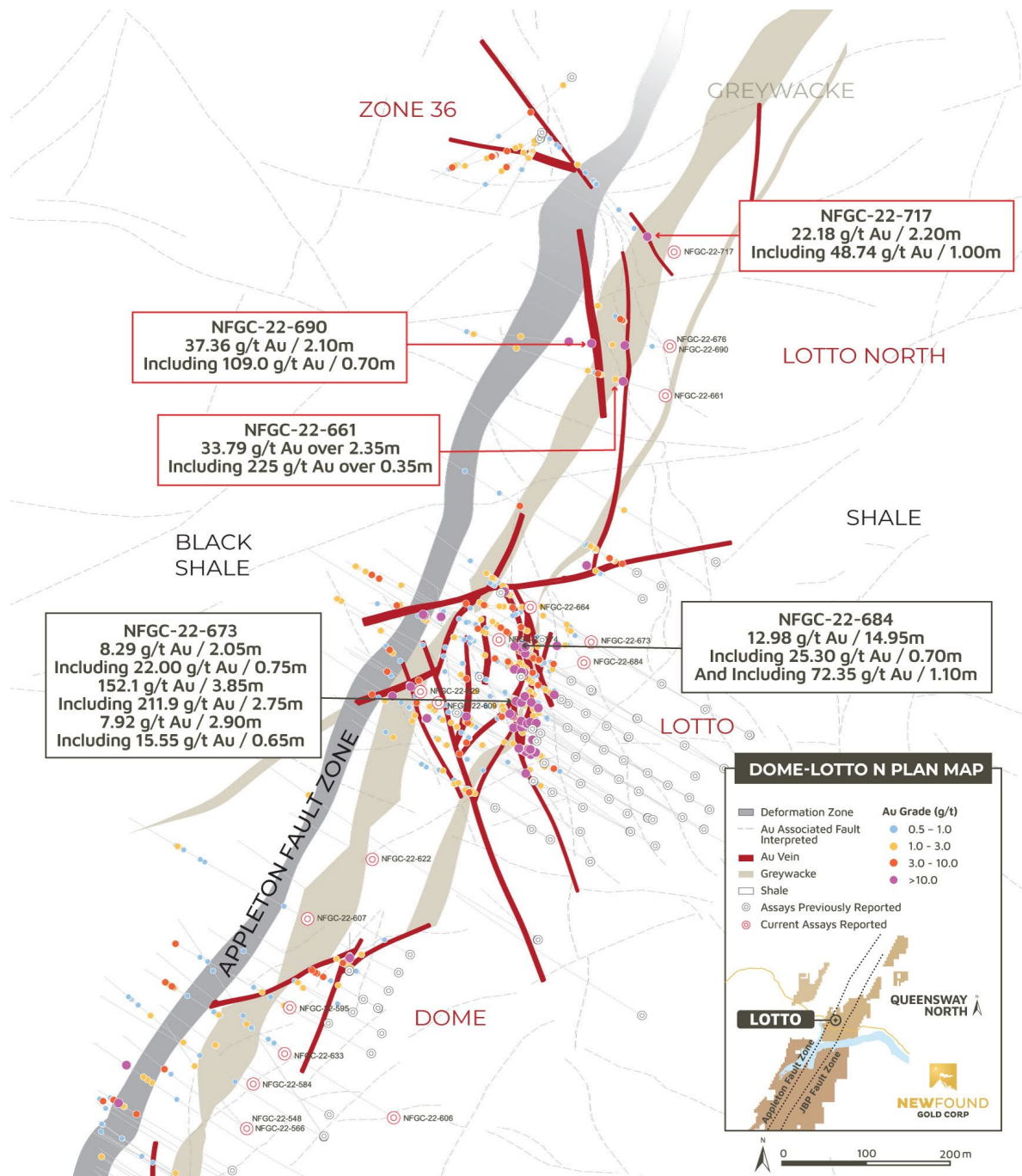
Queensway Project – Dome- Lotto North Plan View Map (November 2, 2022)
